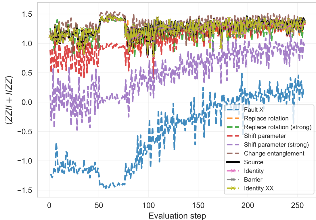
Symmetry Observable Evolution
