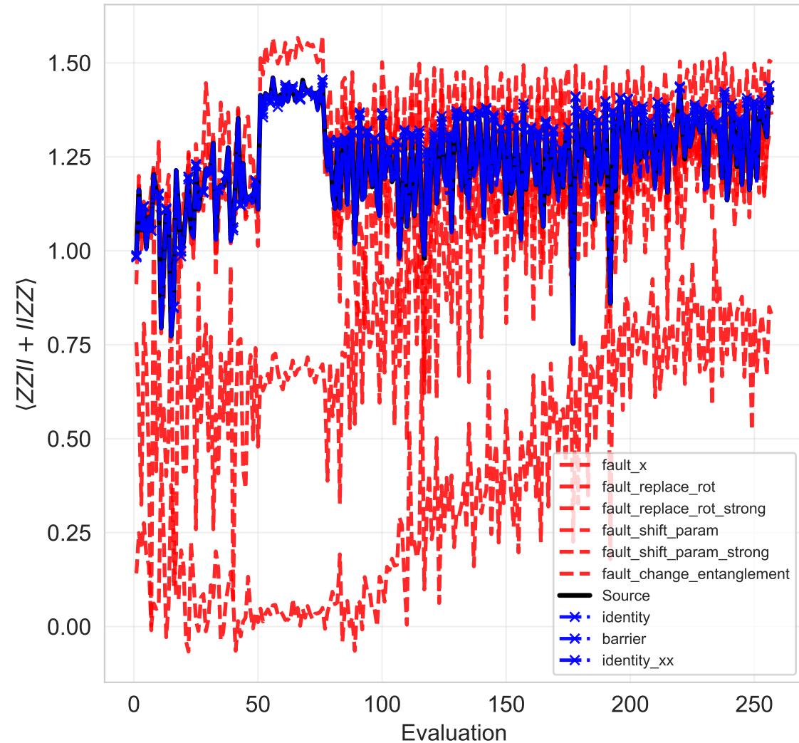
Noisy Symmetry Evolution
