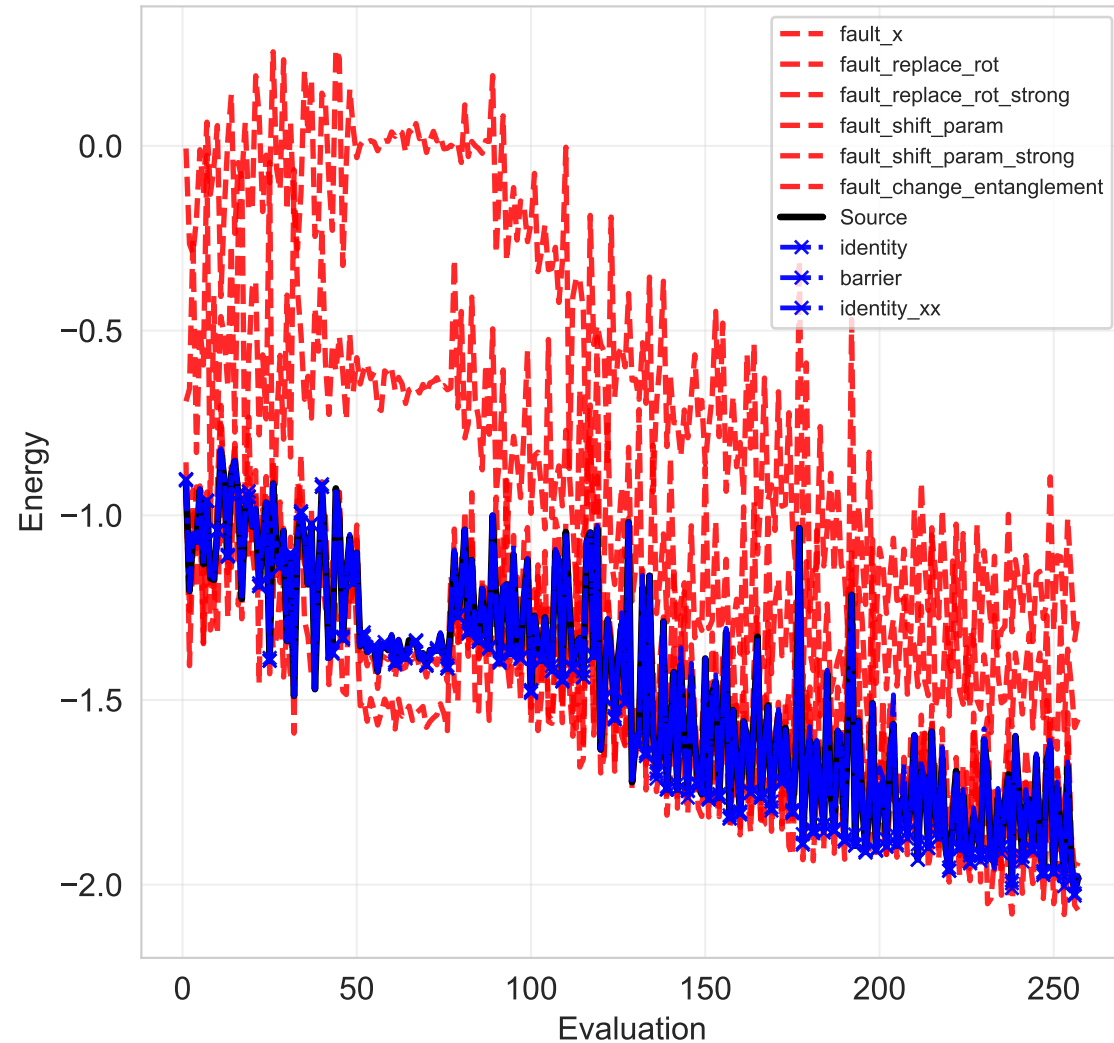
Noisy Energy Convergence
