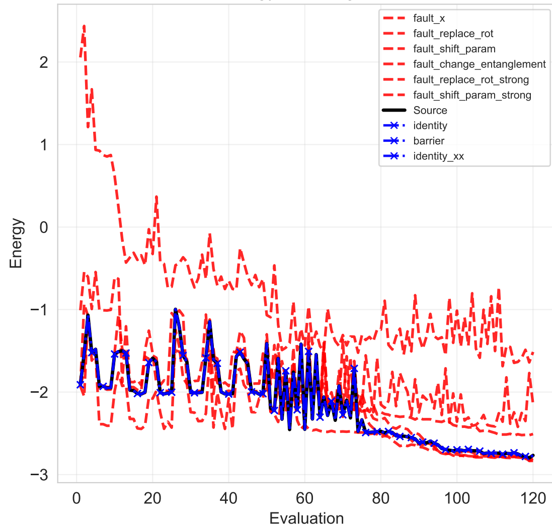
Energy Convergence
