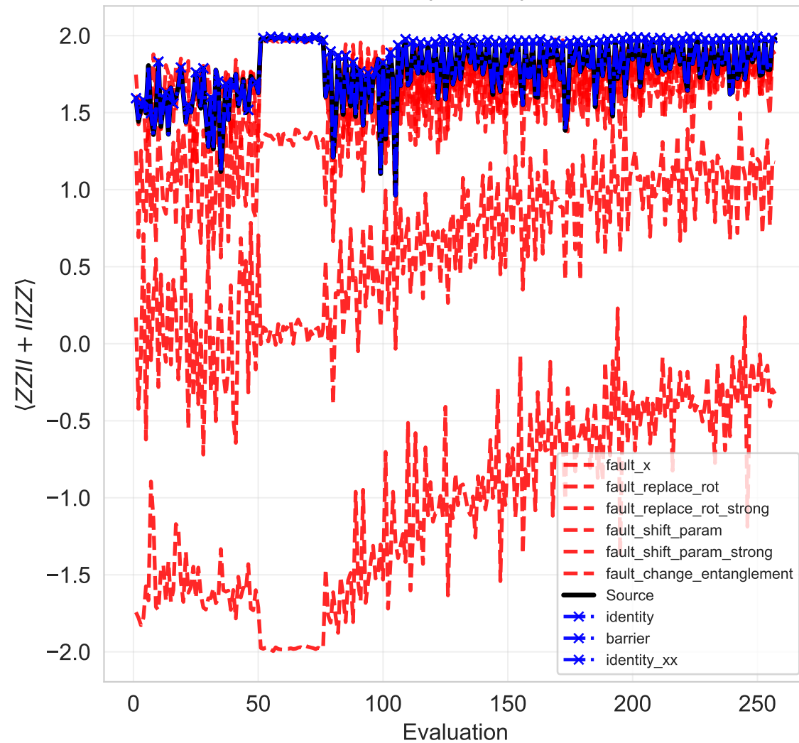
Shot-Based Symmetry Evolution
