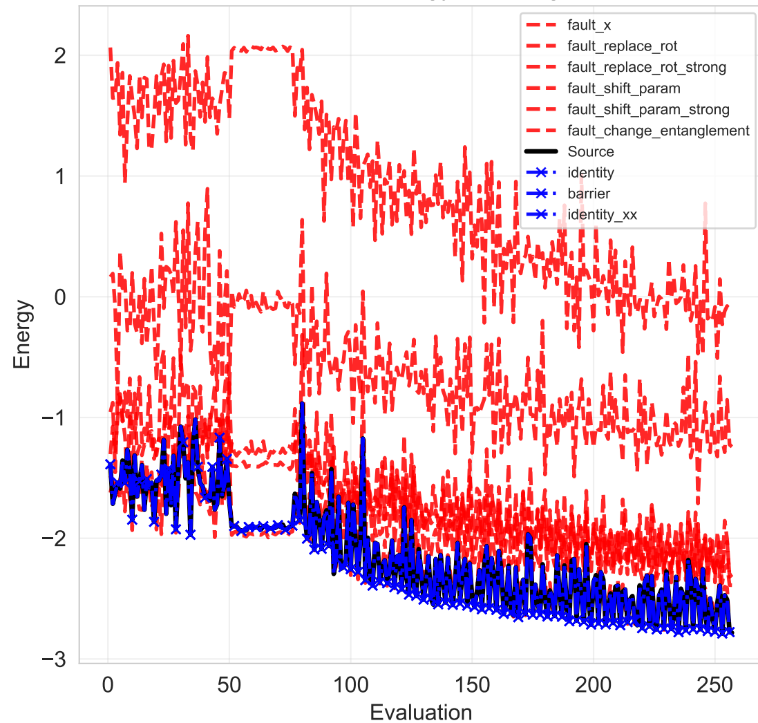
Shot-Based Energy Convergence
