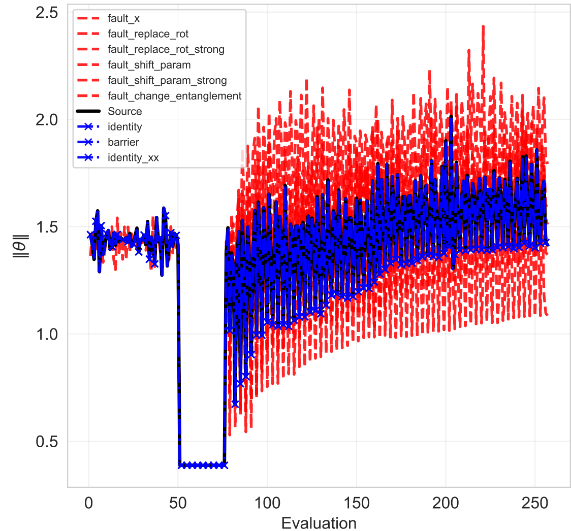
Shot-Based Parameter Norm Evolution
