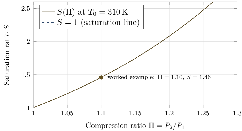
Figure 2. Predicted saturation ratio S as a function of compression ratio \Pi at T_0 = 310\text{ K} , \gamma = 1.4 (Eq. 18). The worked example of Sec. 6 ( \Pi = 1.10 , S = 1.46 ) is marked. The supersaturation threshold S = 1 is shown as a dashed line; any \Pi > 1 produces supersaturation, with rapid growth above \Pi \approx 1.05 .
