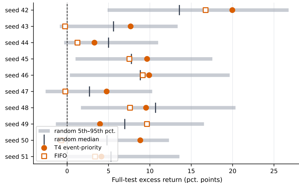
SPY: T4 vs FIFO vs 1,000 random allocations
