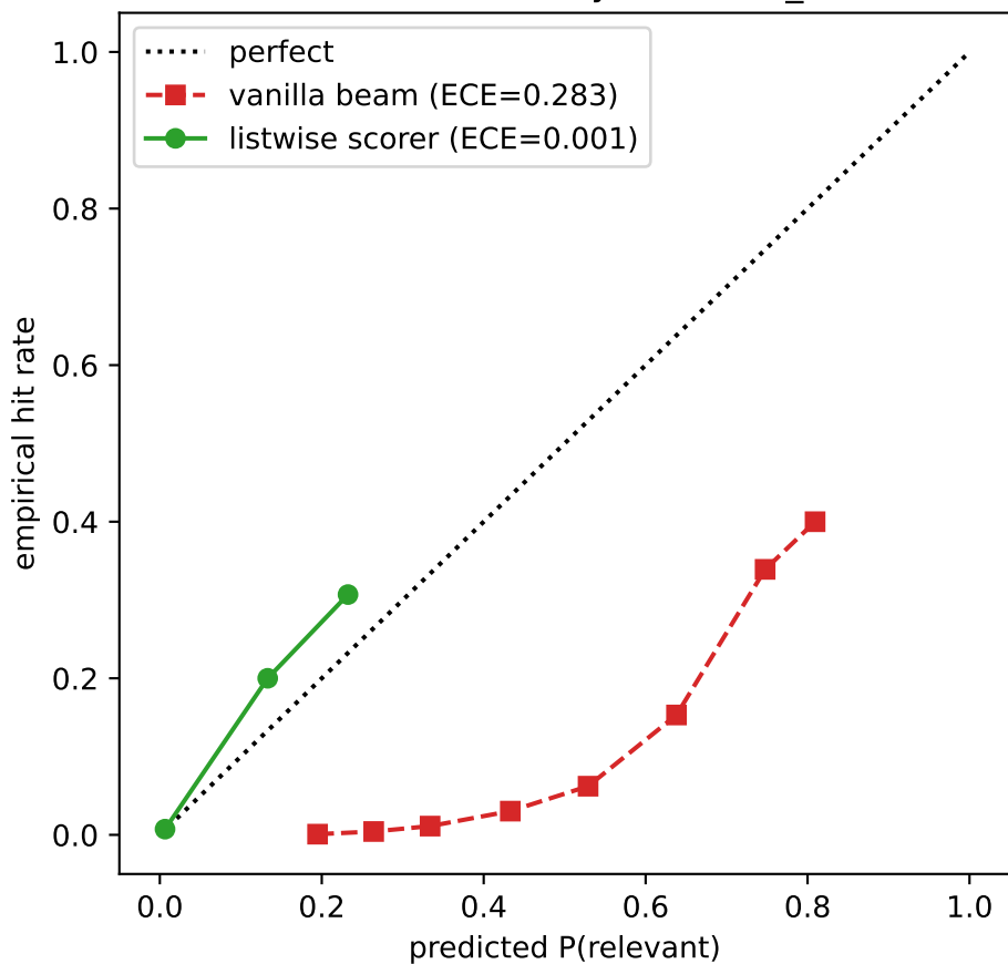
Per-candidate reliability (baseline_retrain)
