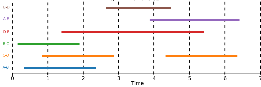
FIGURE 2.7: Illustration of two common representations of temporal networks. (a) Contact sequence: each interaction is instantaneous and recorded as a triplet (i, j, t) . (b) Interval graph: each interaction spans a time interval and is recorded as a quadruplet (i, j, t_{\text{start}}, t_{\text{end}}) .
