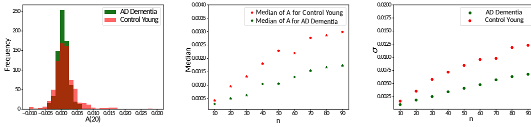
FIGURE 6.3: Summary Statistics of Non-Parametric Expansion A(n) for Control and AD Dementia. (Left) Frequency histogram of A(n = 20) , extracted from the network trajectory of a control young individual (red bars) and a patient diagnosed with AD Dementia (green bars). (Middle) Median of the population of A as a function of the monitoring time n , comparing a control young individual (red points) to a patient diagnosed with AD Dementia (green points). The control individual systematically exhibits a larger median, suggesting that this metric may serve as a distinguishing parameter between cases. (Right) Same as the middle panel, but using the standard deviation \sigma(A(n)) of the population as the metric.
