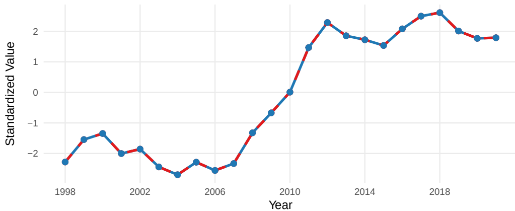
08.PredBirdNCC_b_0_smoothed
