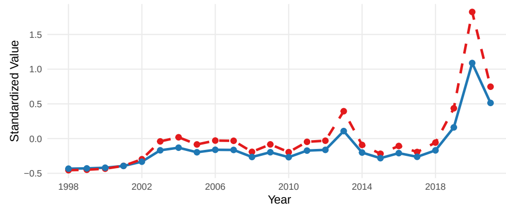
05.ForageFishNCC_0_smoothed
