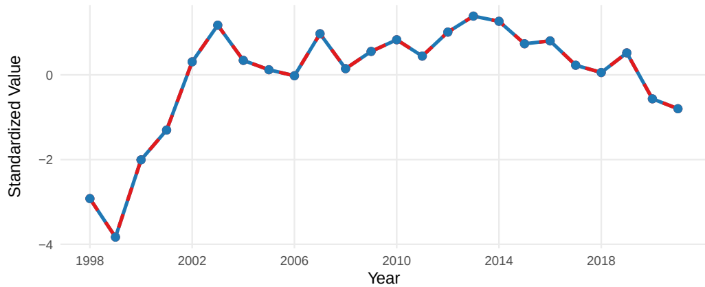
08.PredBirdNCC_DFA1
