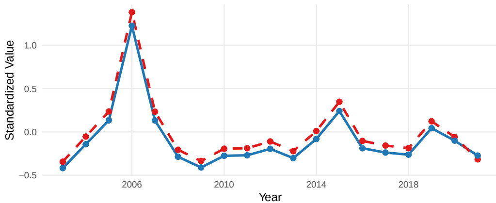
09.PredFishNCC_b_DFA1
