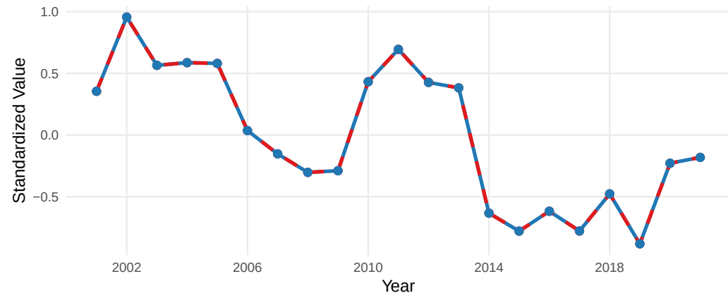
01.ZooPreyNCC_NHL_2_smoothed
