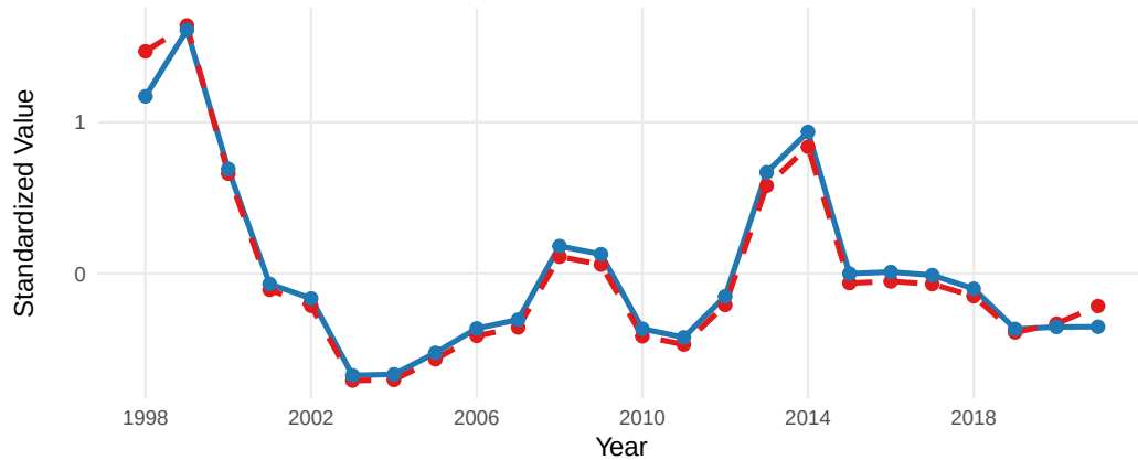
13.FishPreyAK_b_DFA1
