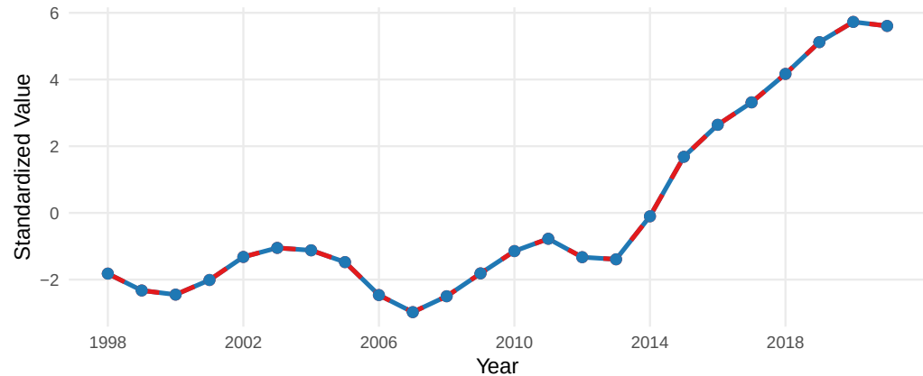
14.CompAK_1_smoothed
