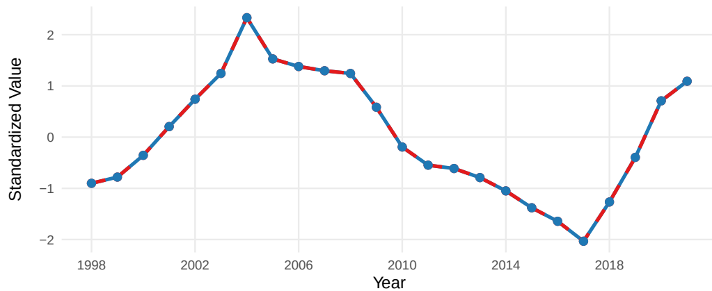
02.CompJellyNCC_DFA1
