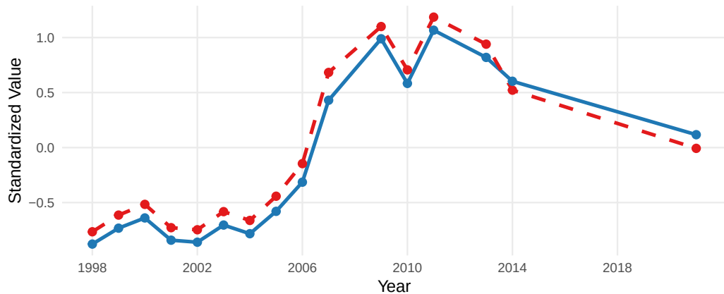
12.ZooPreyAK_0_smoothed
