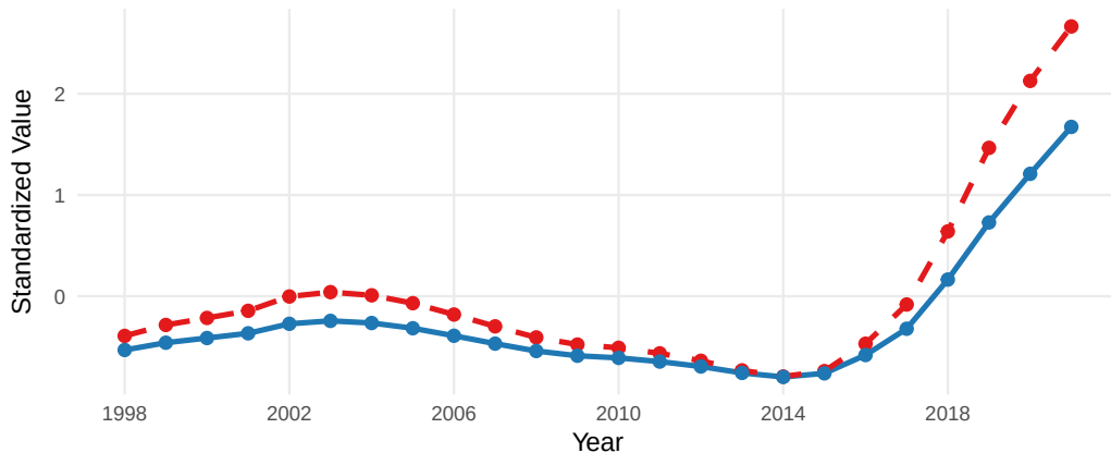
15.PredFishAK_3_smoothed
