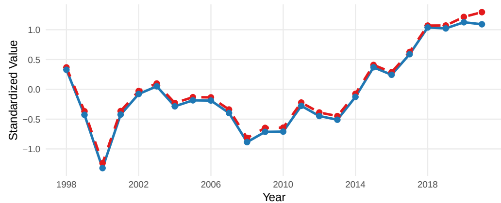
13.FishPreyAK_b_0_smoothed
