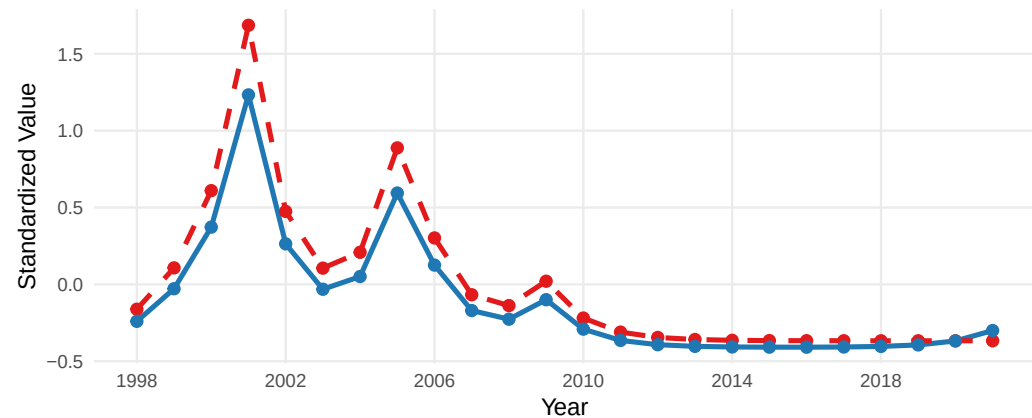
13.FishPreyAK_b_2_smoothed
