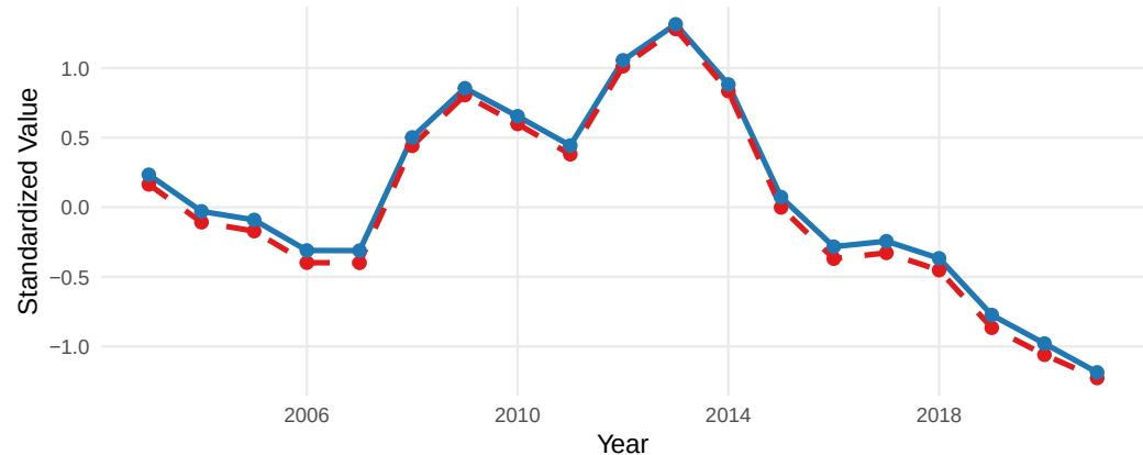
15.PredFishAK_b_2_smoothed
