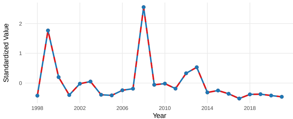
08.PredBirdNCC_b_1_smoothed
