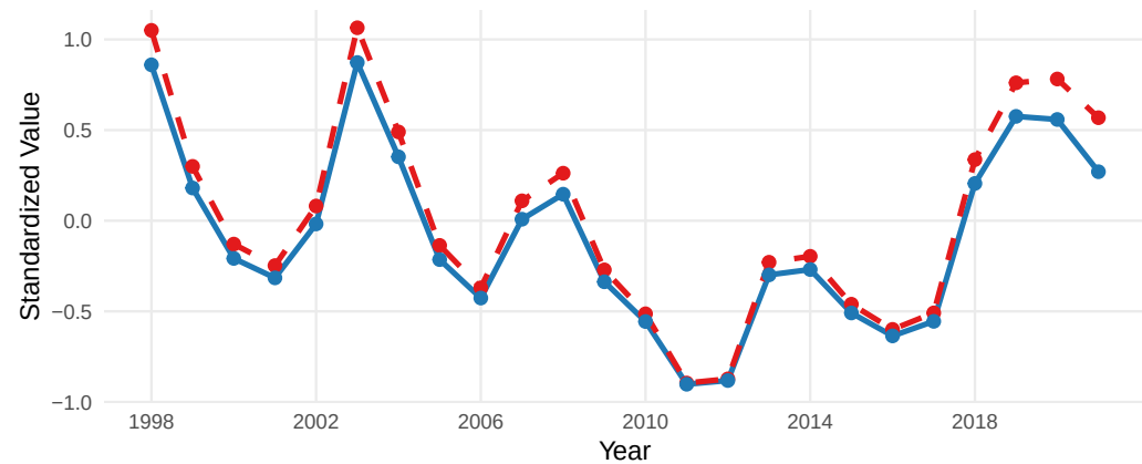
06.Cond1NCC_0_smoothed
