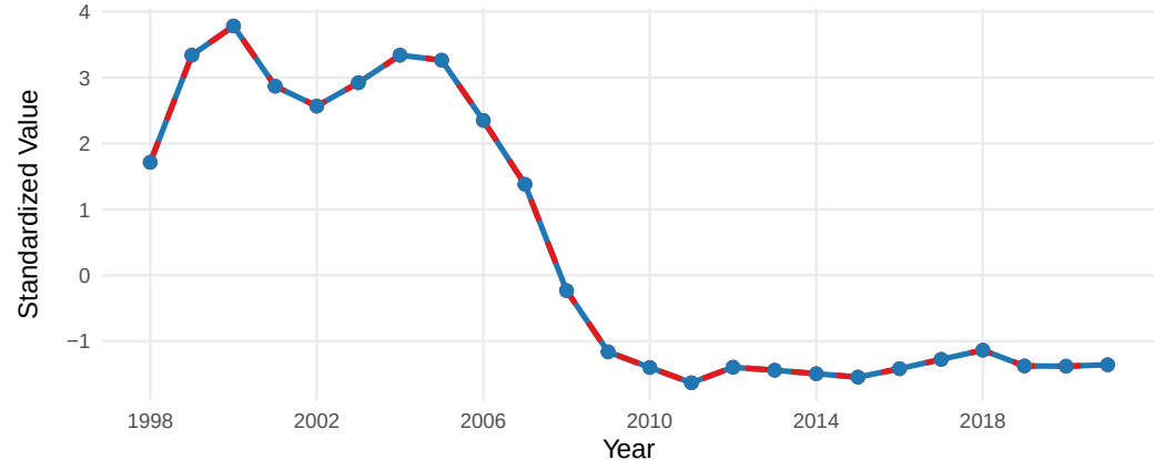
15.PredFishAK_b_DFA1
