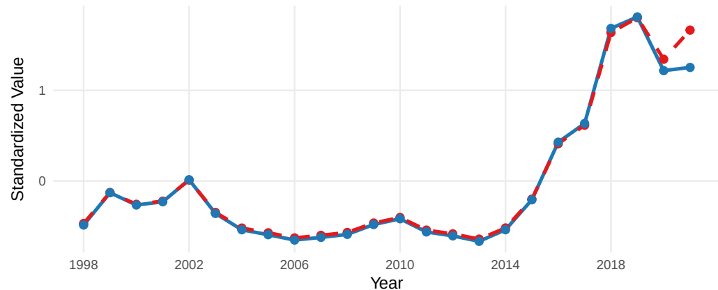
15.PredFishAK_4_smoothed
