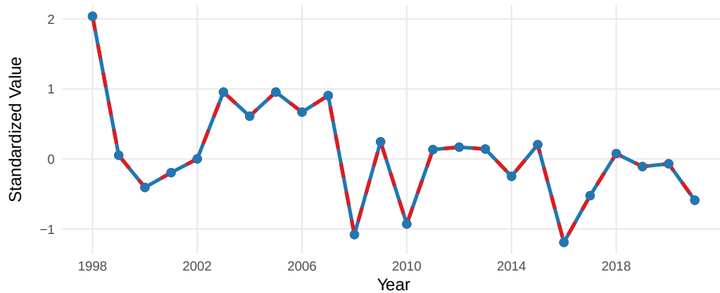
04.CompFishNCC_1_smoothed
