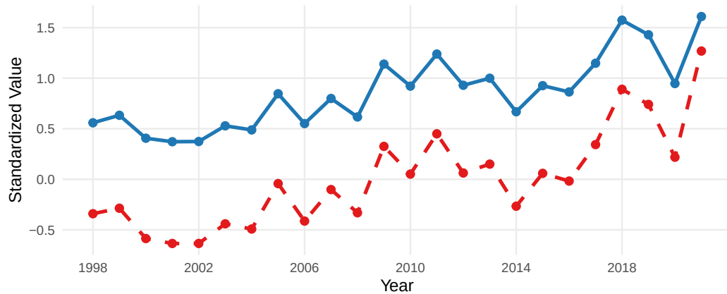
14.CompAK_0_smoothed
