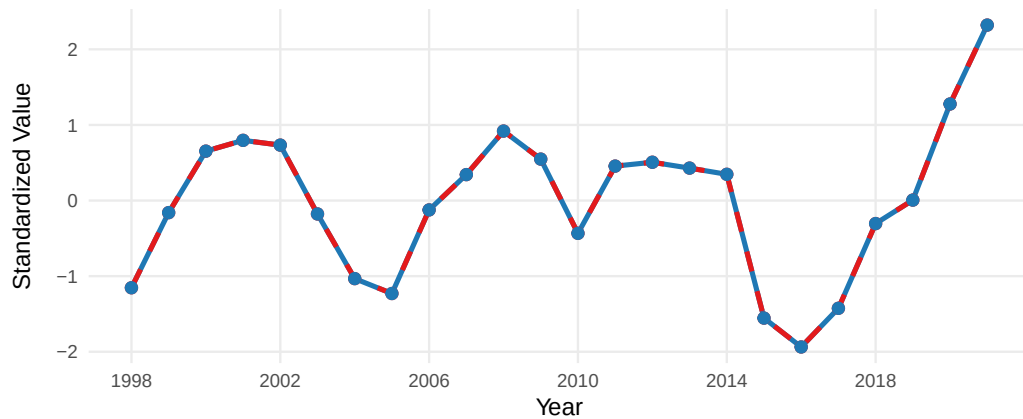
01.ZooPreyNCC_WPbirds_1_smoothed
