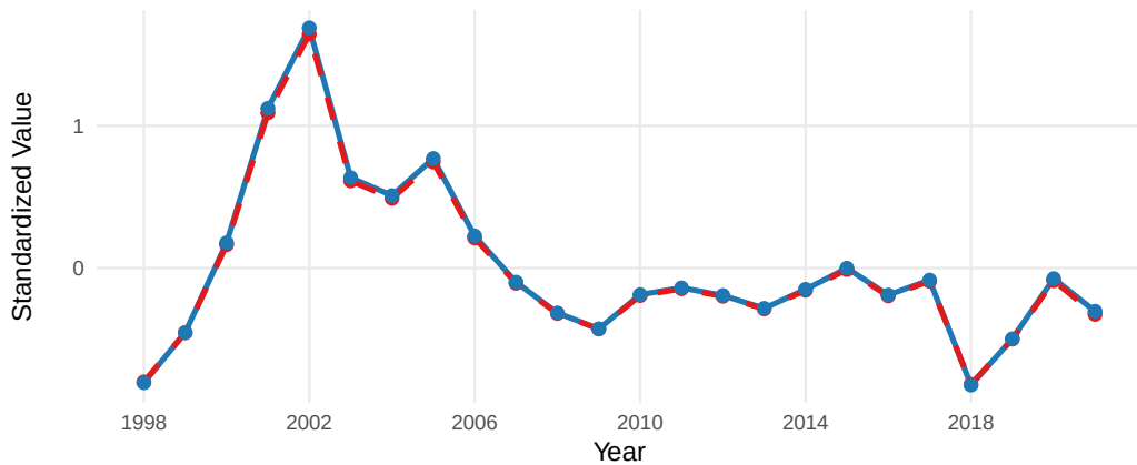
10.PredMammalNCC_DFA1
