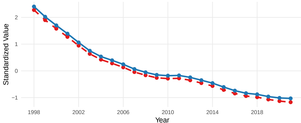
15.PredFishAK_b_1_smoothed
