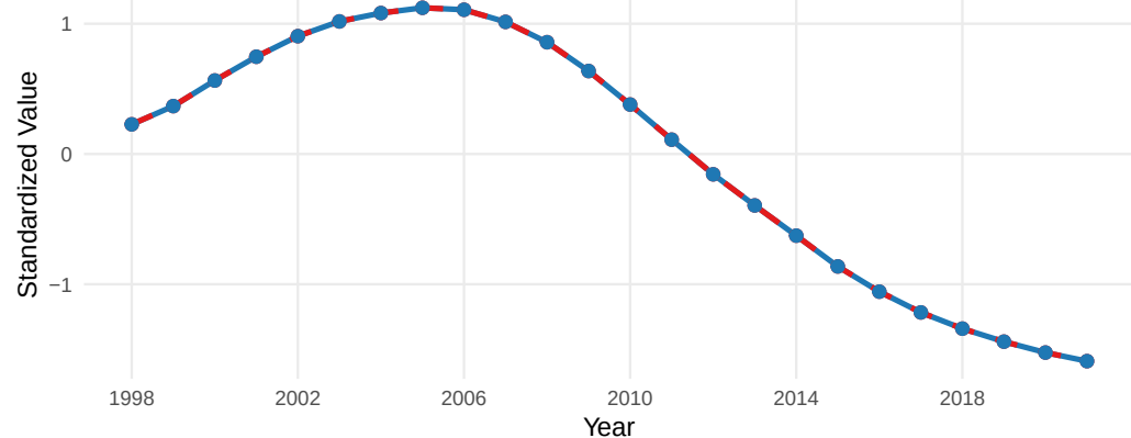
15.PredFishAK_2_smoothed
