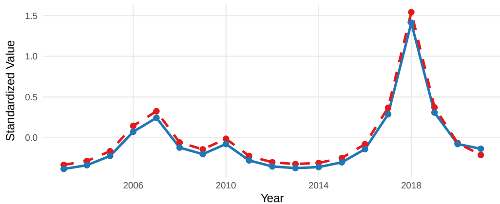
09.PredFishNCC_DFA1
