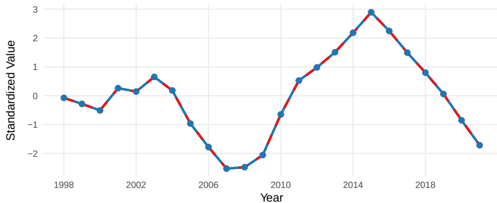
13.FishPreyAK_b_1_smoothed
