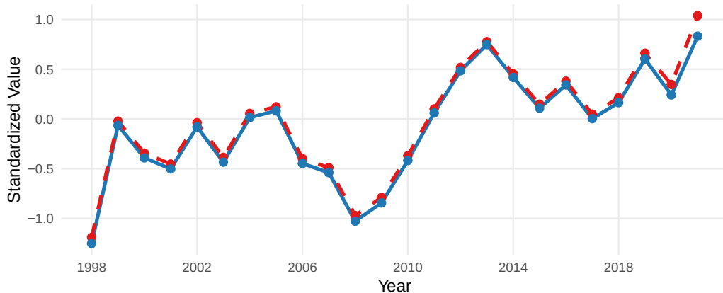
01.ZooPreyNCC_JSOES_DFA1
