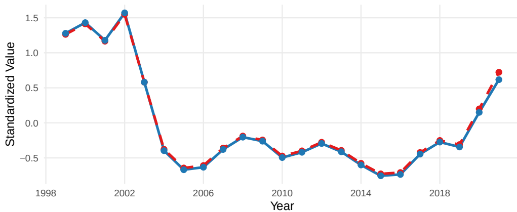
06.Cond1NCC_1_smoothed
