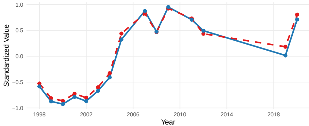
10.PredMammalNCC_1_smoothed
