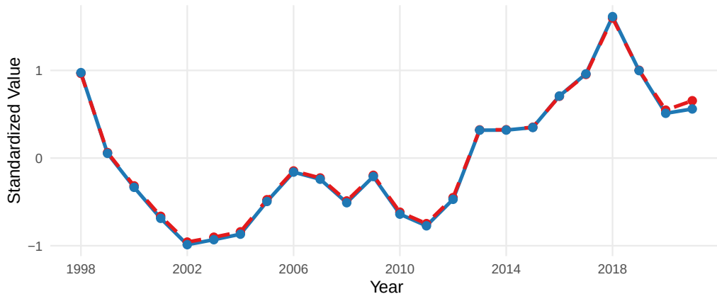
15.PredFishAK_b_3_smoothed
