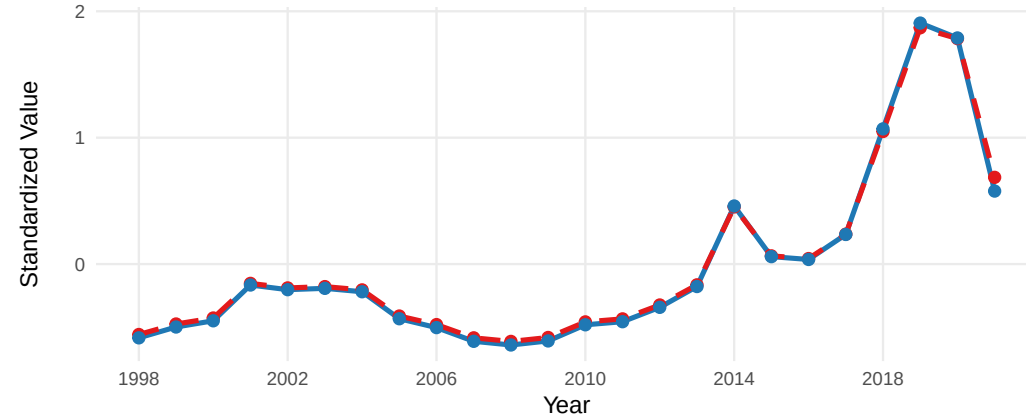
04.CompFishNCC_2_smoothed
