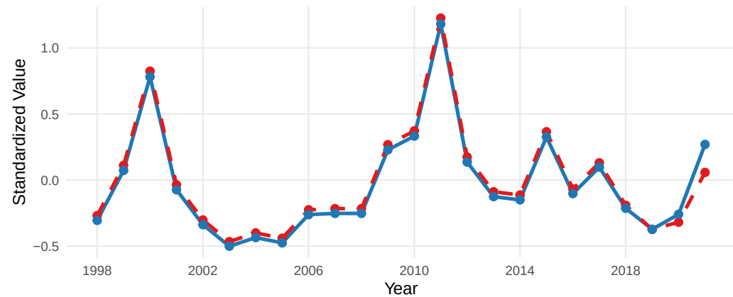
03.FishPreyNCC_0_smoothed
