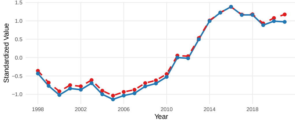
04.CompFishNCC_smoothed
