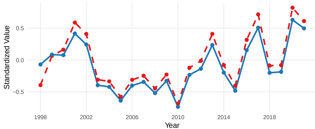
12.ZooPreyAK_DFA1
