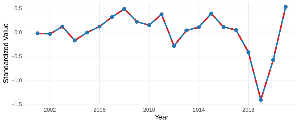
01.ZooPreyNCC_NHL_1_smoothed
