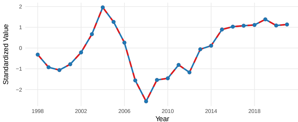
10.PredMammalNCC_0_smoothed
