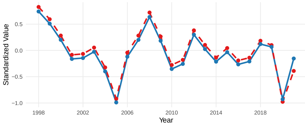
08.PredBirdNCC_b_2_smoothed
