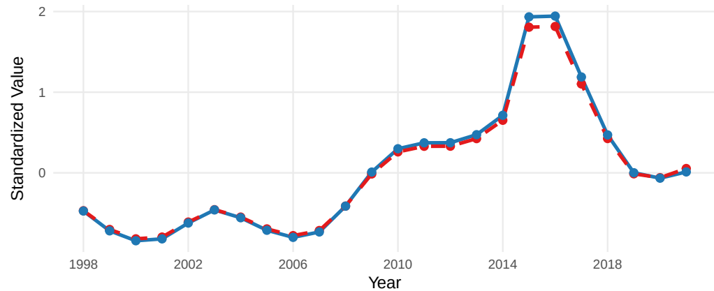
13.FishPreyAK_DFA1
