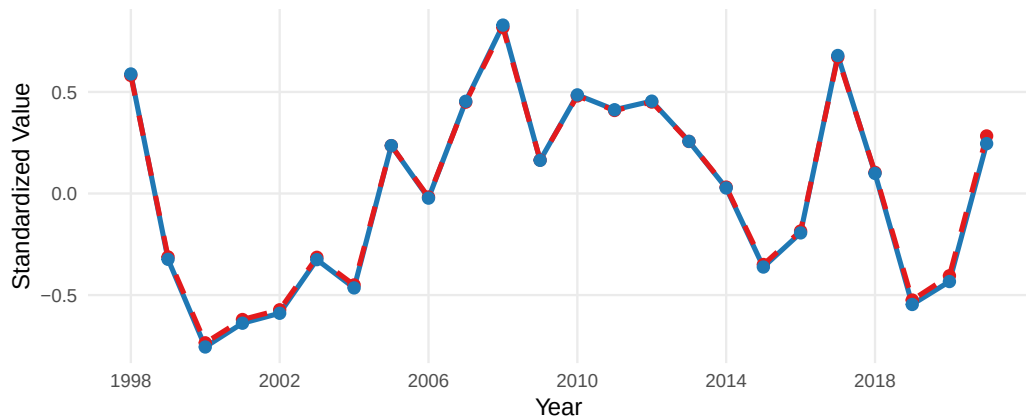
11.PredMammalSmolt_0_smoothed
