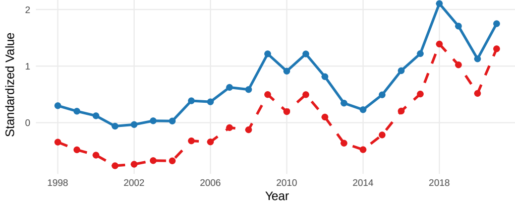
15.PredFishAK_1_smoothed
