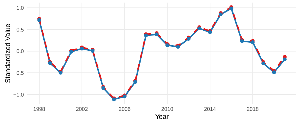
01.ZooPreyNCC_WPbirds_smoothed
