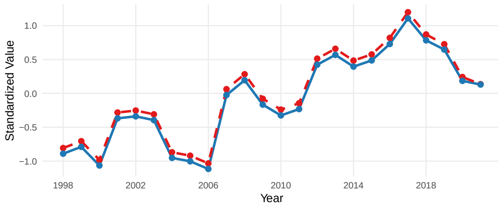
05.ForageFishNCC_DFA1
