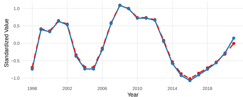
01.ZooPreyNCC_NHL_0_smoothed
