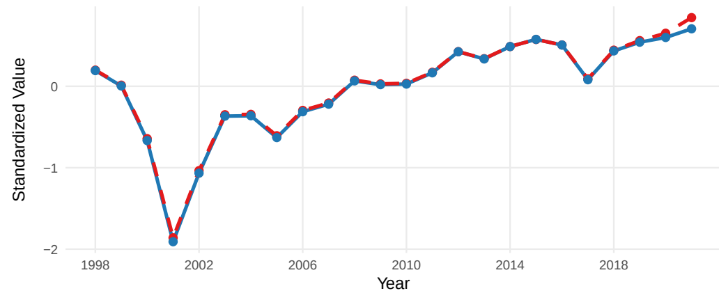
06.Cond1NCC_2_smoothed
