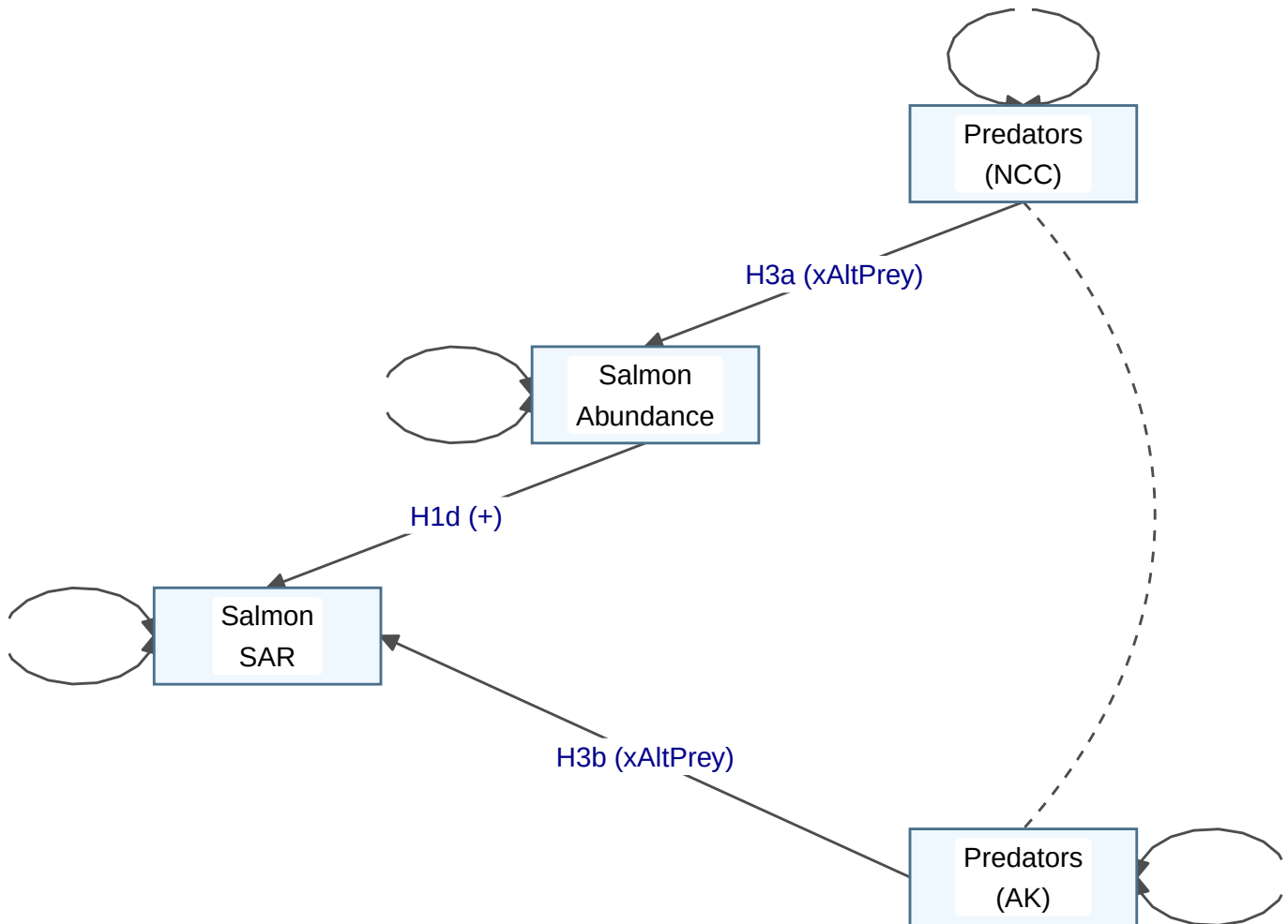
DAG 1D: Two-Stage Interaction Model
