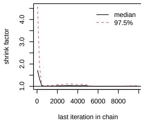
rOM_ClxHorse.1.
