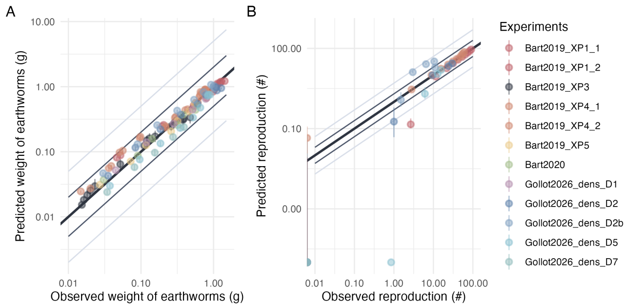
Figure 2.12: Predicted versus observed values of weight and reproduction. Points are colored by experimental conditions. Grey and light-grey lines represent the 2-folds and 5-fold changes, respectively. The bold black line represents the identity line.
