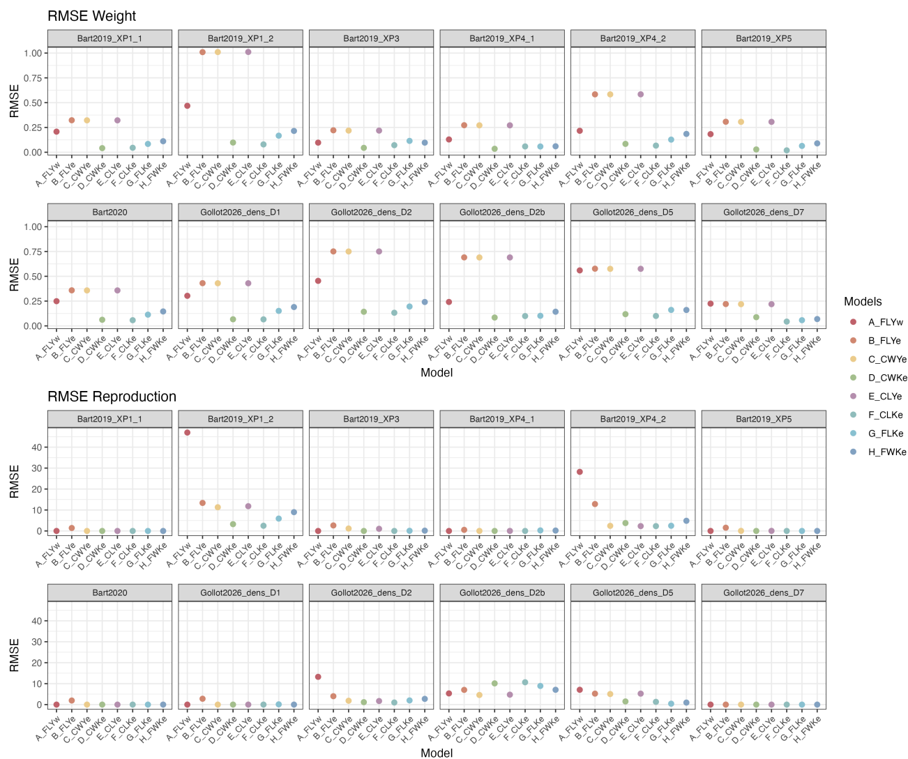
Figure 2.27: RMSE for Weight and Reproduction per experiment for each tested model.
