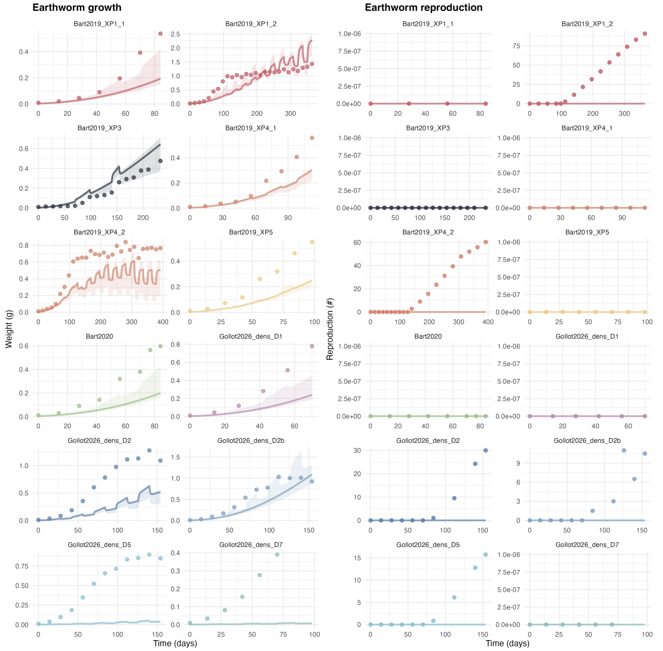
Figure 2.2: Observed and predicted growth and reproduction trajectories for each experiment . Points represent observed data, solid lines represent estimated model trajectories, and ribbons indicate the 95% credibility intervals.
