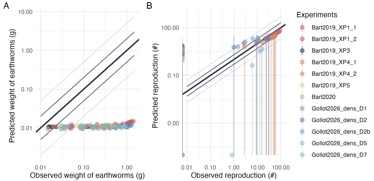
Figure 2.4: Predicted versus observed values of weight and reproduction. Points are colored by experimental conditions. Grey and light-grey lines represent the 2-folds and 5-fold changes, respectively. The bold black line represents the identity line.
