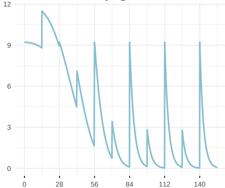
Organic_matter
