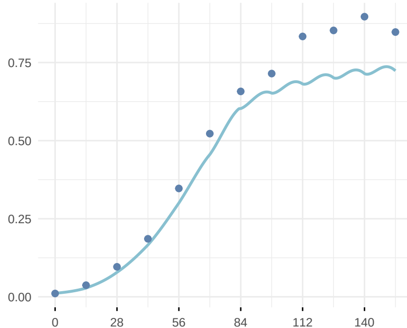
Weight
