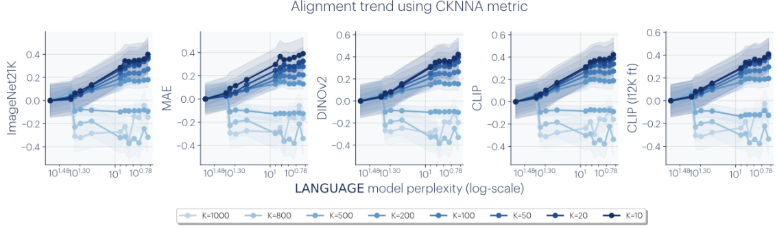
Figure 10. Cross-modal alignment increases locally: Alignment trend when varying the top- k nearest neighbors in the CKNN metrics (Eqn. 18). We center alignment score to the smallest language model and divide the total trend by the standard deviation. When k = 1024 , we recover the original CKA metric, and when k < |\mathcal{X}| it closely resembles the mutual nearest-neighbor metric m_{NN} . Each line represents the average of all LLM models for a specific k . As we decrease k , the alignment becomes more pronounced.
