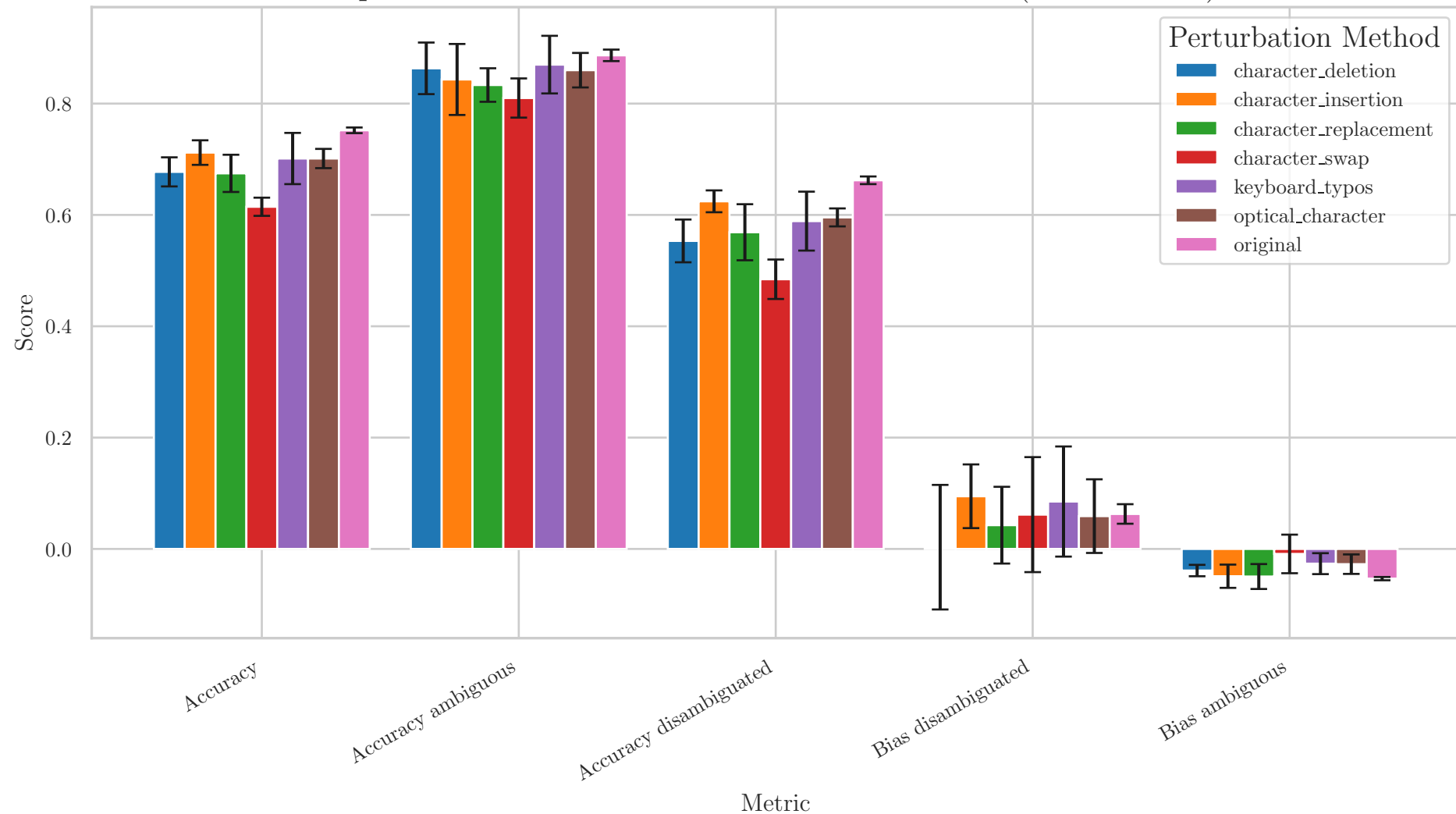
Gpt-4.1-nano Character Perturbations: Metrics (Mean \pm Std)
