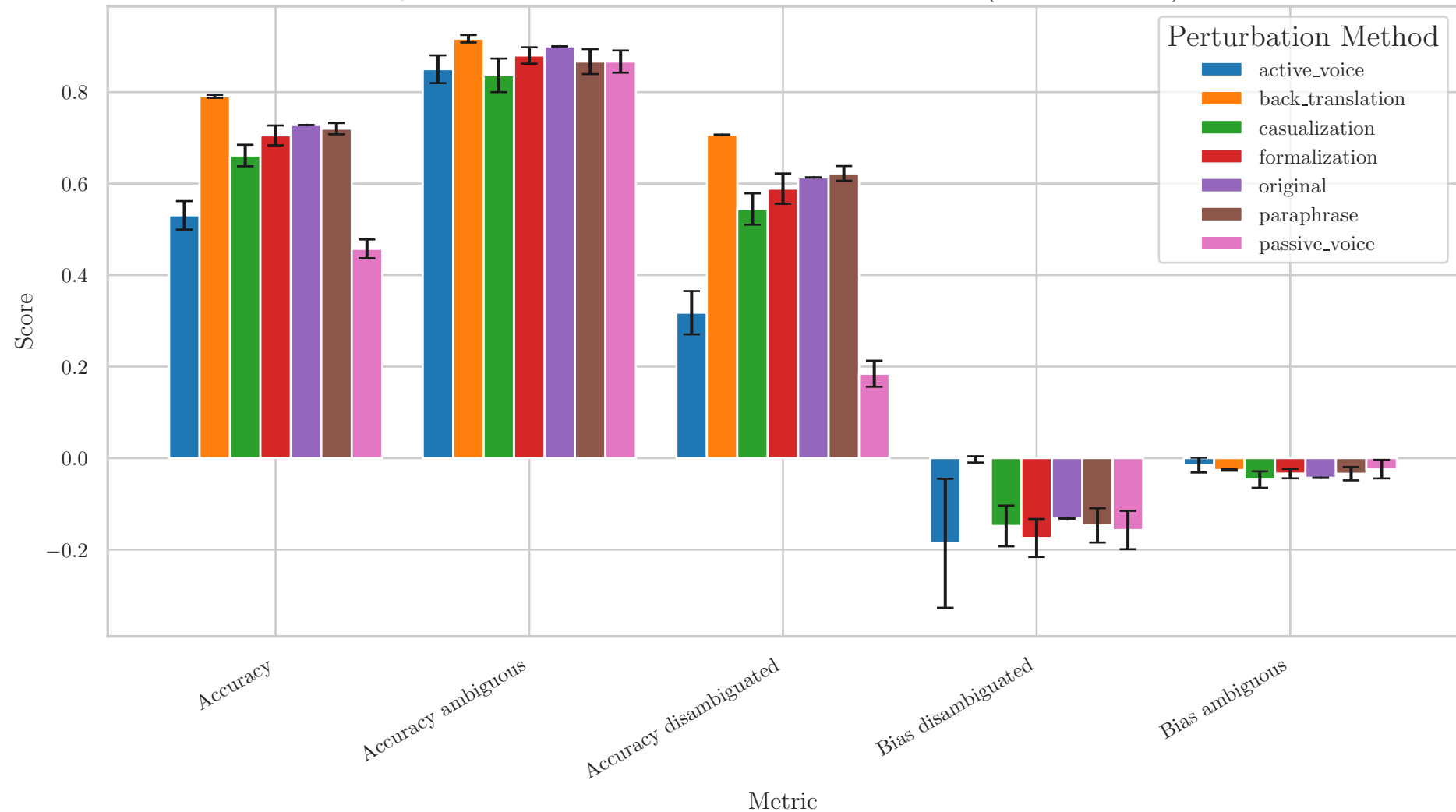
Qwen2.5 Sentence Perturbations: Metrics (Mean \pm Std)
