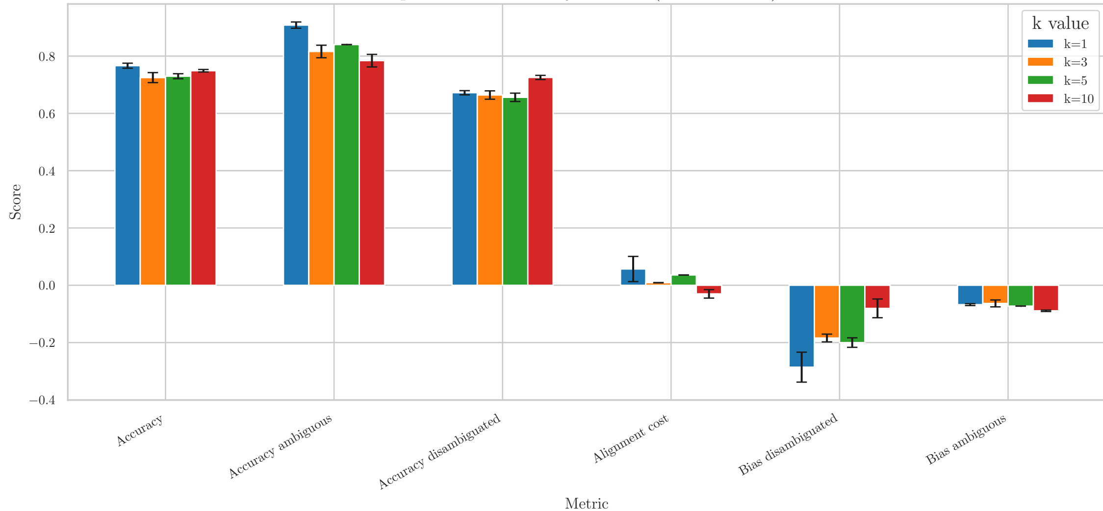
qwen2.5: Metrics by k value (Mean \pm Std)
