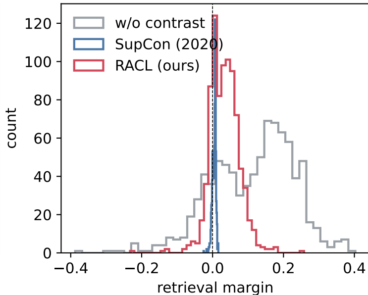
Retrieval-margin distribution
