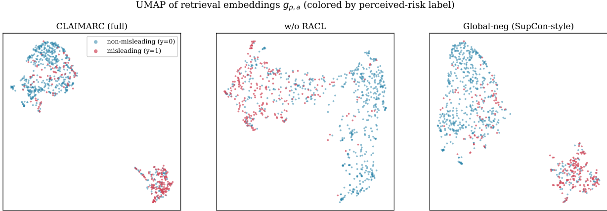
Figure 3: UMAP of the retrieval embedding \mathbf{g}_{p,a} (test), colored by perceived-risk label. The full model (left) isolates the misleading pairs into a detached cluster; removing RACL (middle) collapses the separation.
