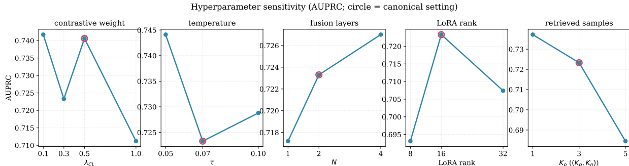
Figure 4: Hyper-parameter sensitivity (AP). Across all five sweeps the score stays inside a narrow band; the canonical configuration (circled) sits on the stable plateau.
