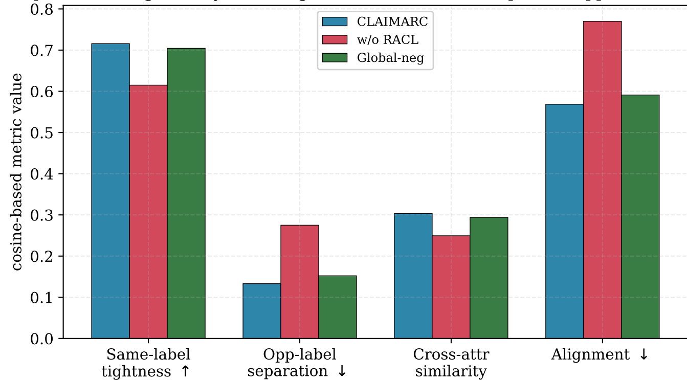
Representation geometry: RACL tightens same-label and separates opposite-label pairs
