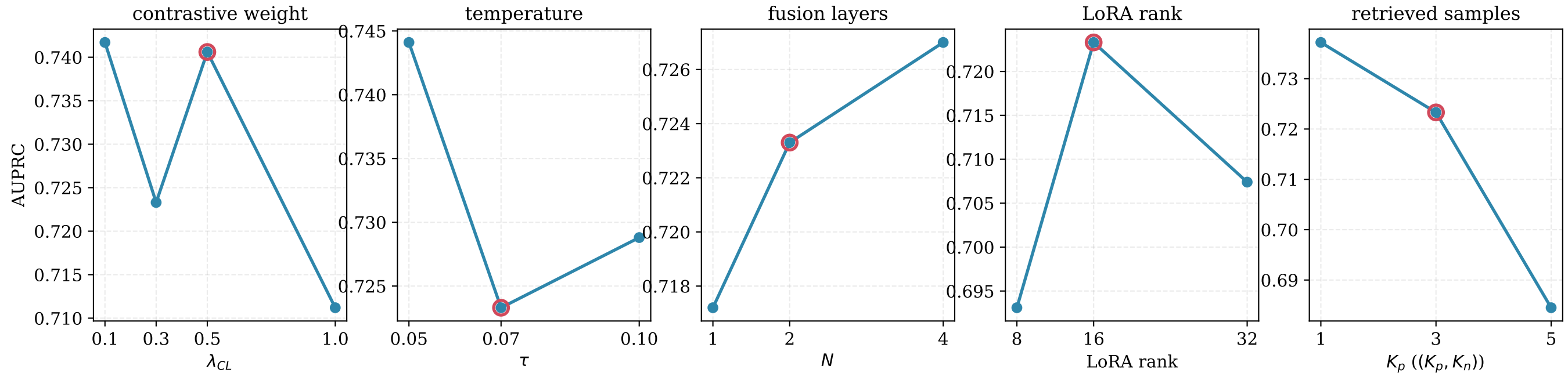
Hyperparameter sensitivity (AUPRC; circle = canonical setting)
