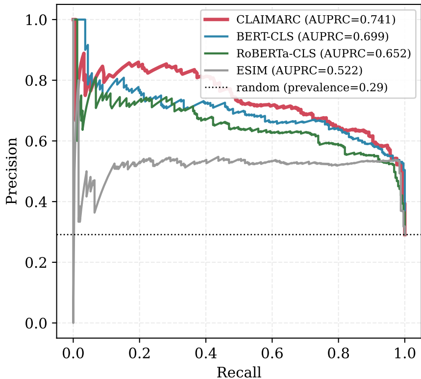
(a) Precision-Recall
