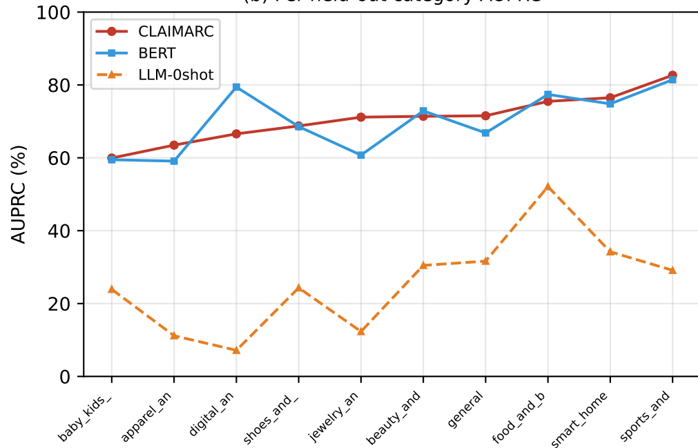
(b) Per held-out category AUPRC
