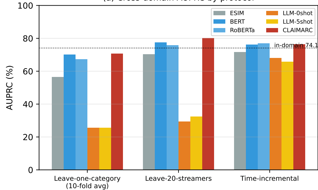
(a) Cross-domain AUPRC by protocol
