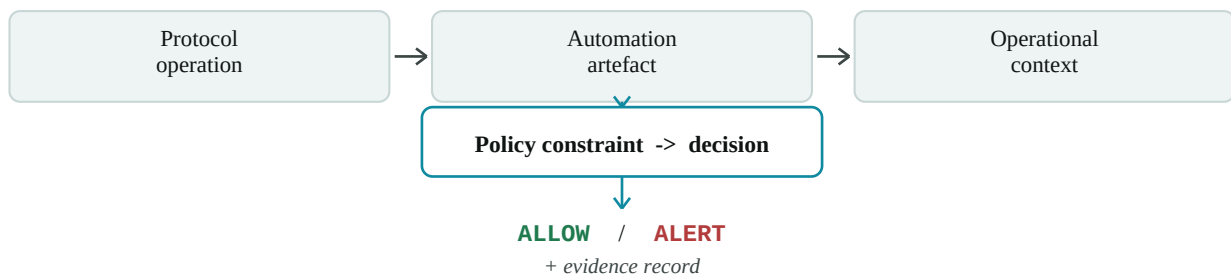
Figure 1: The action-evaluation chain. An action is characterised along three descriptive dimensions and evaluated against policy to yield a decision and an evidence record. The chain is protocol-agnostic; Modbus/TCP is the first instantiation.
