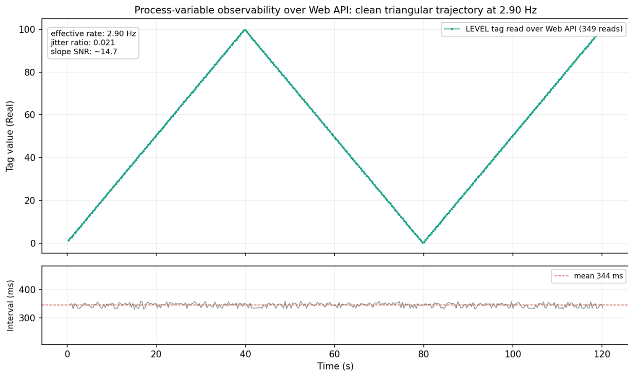
Figure 4. The ramp trajectory read over the Web API (349 reads, upper panel), and the inter-read interval over the same period (lower panel). The trajectory is clean and the sampling near-regular, at an effective rate of 2.9 Hz with a jitter ratio of 0.02.
