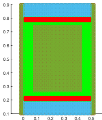
alphaShape
