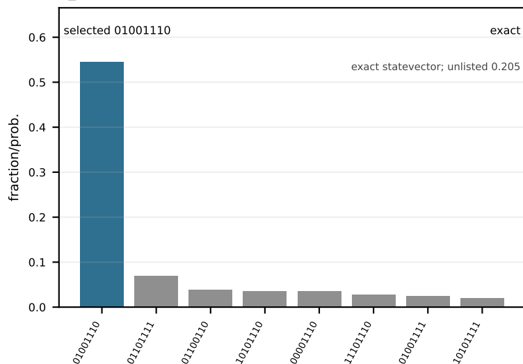
8_11 (easy, q=8)
