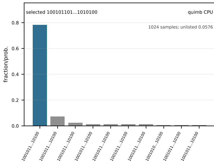
8_11 (easy, q=8)
