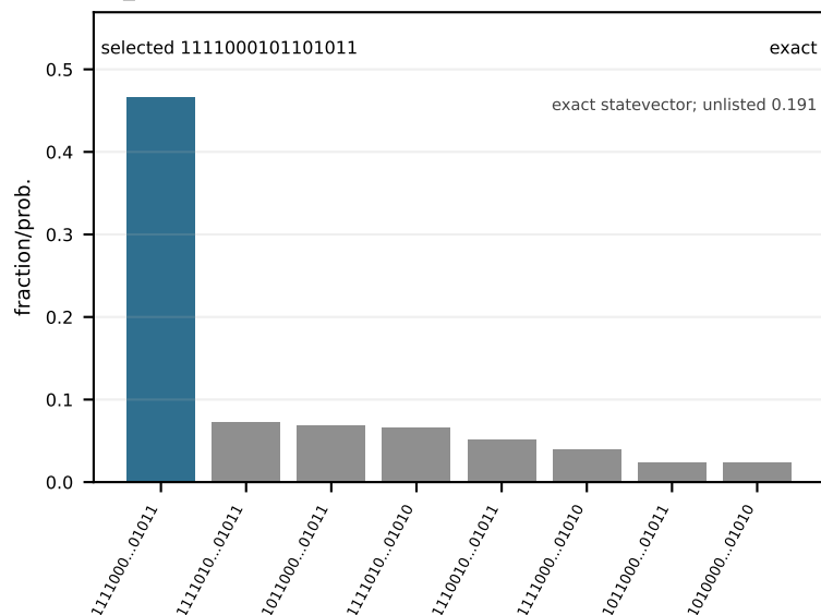
16_12 (easy, q=16)
