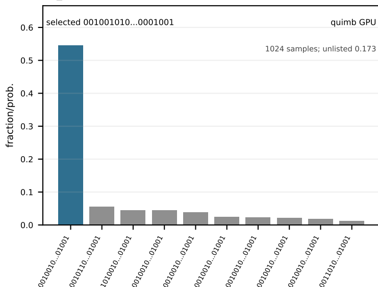
40_17 (easy, q=40)
