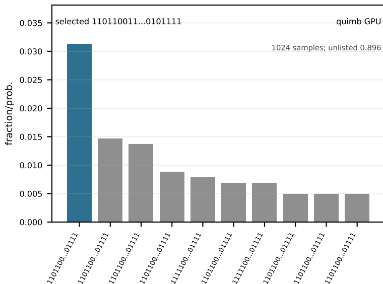
40_17 (easy, q=40)
