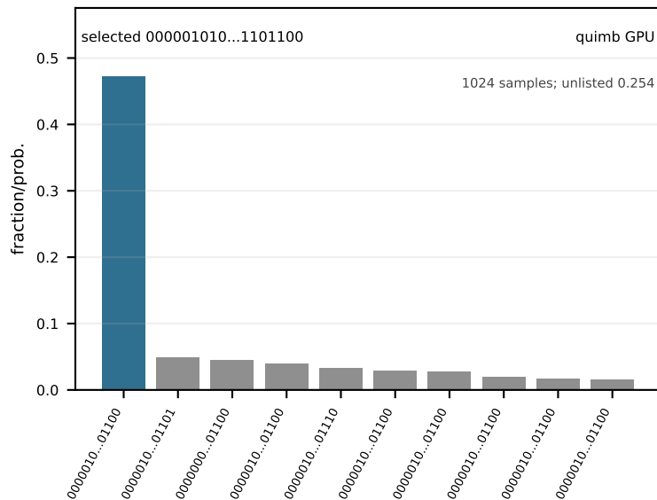
40_16 (easy, q=40)
