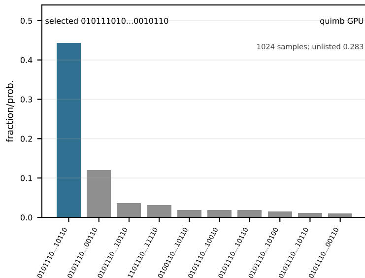
40_18 (easy, q=40)
