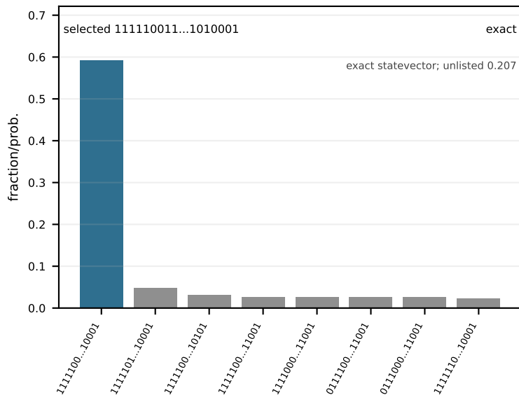
36_15 (easy, q=36)
