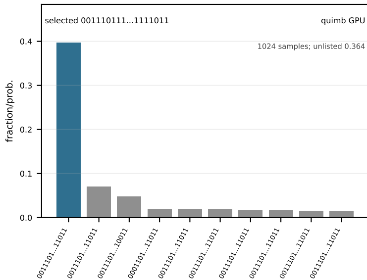
8_27 (moderate, q=8)
