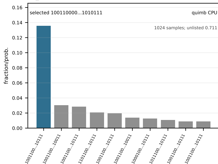
32_30 (moderate, q=32)
