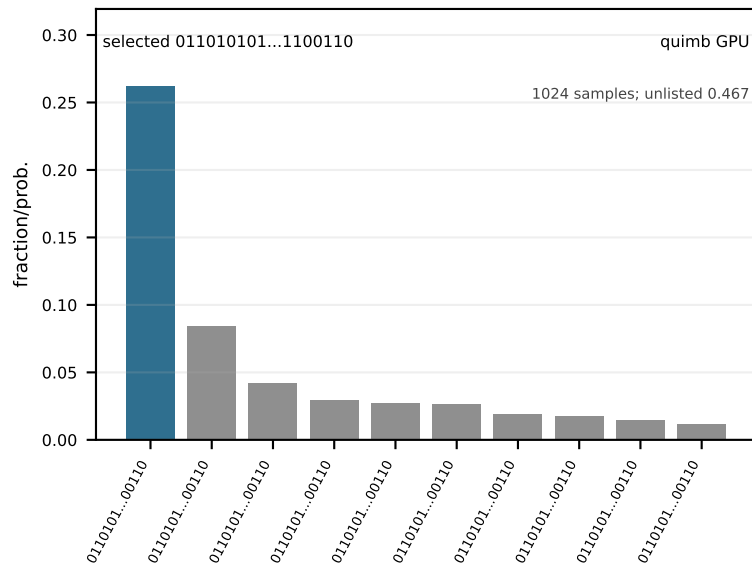
16_28 (moderate, q=16)
