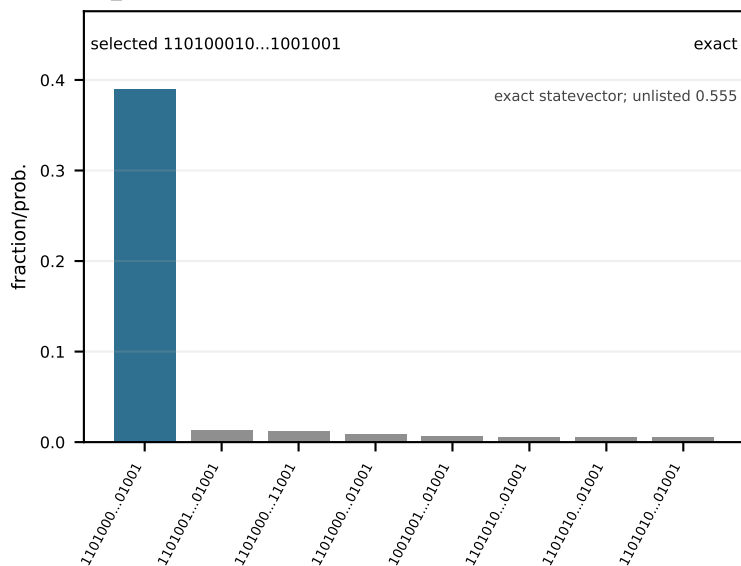
24_29 (moderate, q=24)
