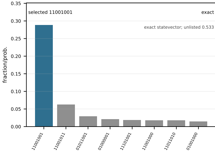
8_27 (moderate, q=8)
