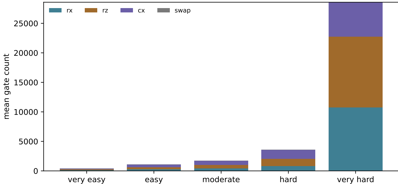
Mean QASM size by difficulty
