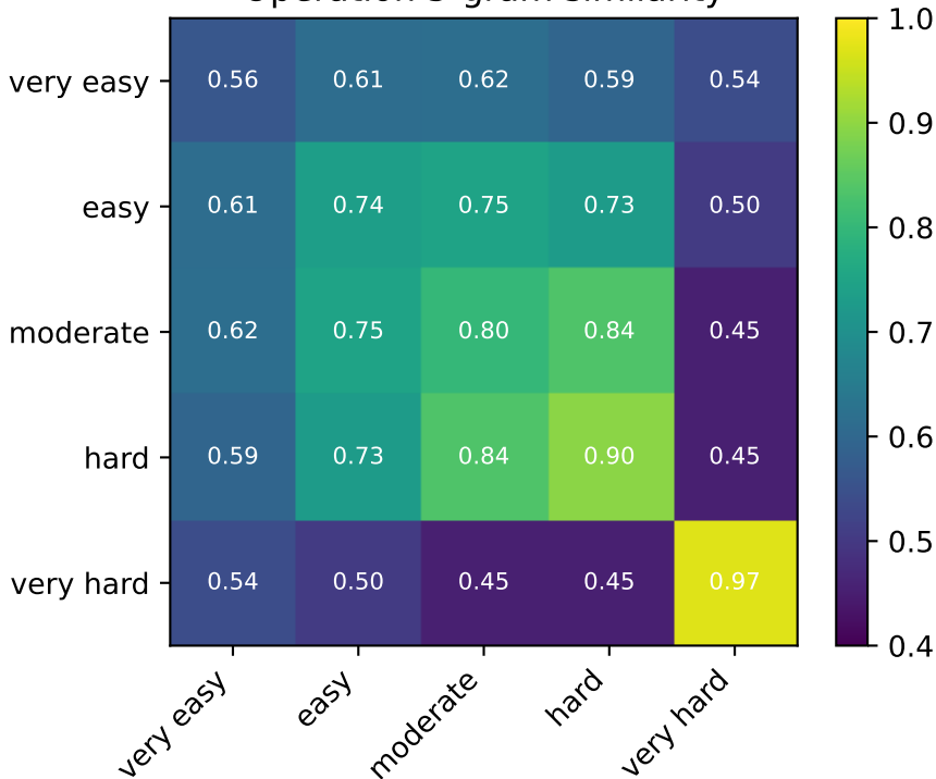
Operation 5-gram similarity
