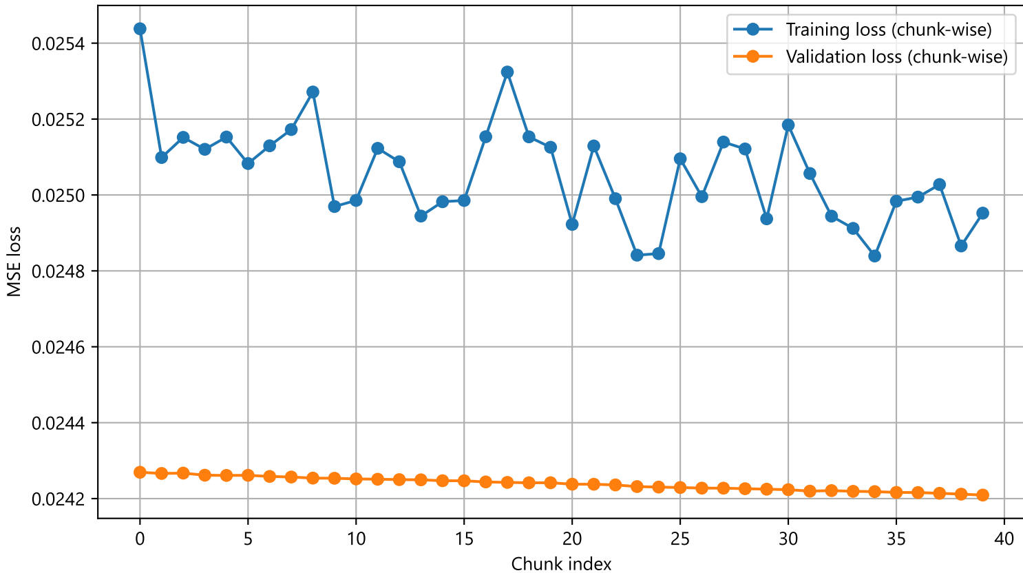
Training vs Validation Loss (chunk-wise) Well-adjusted model (gap < 10%)
