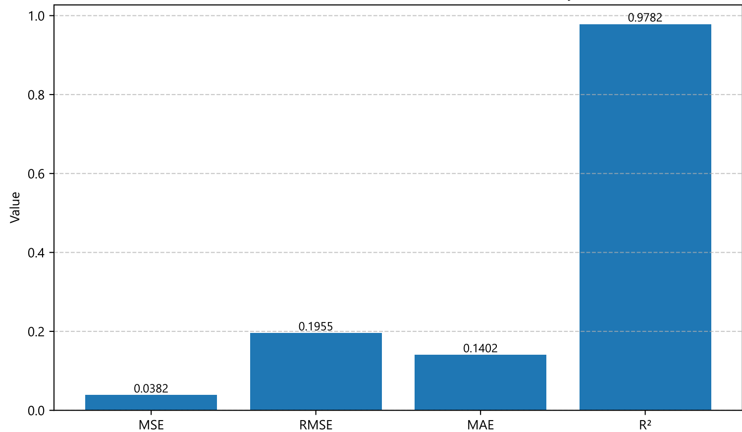
Evaluation Metrics — Quantized INT8 Conv1D Tiny
