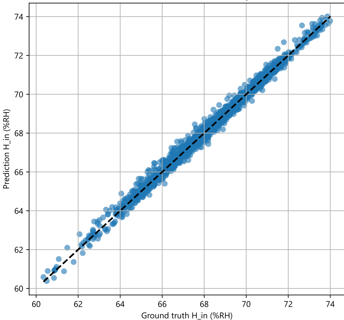
Ground Truth vs Prediction — Humidity (H_in) Quantized INT8 Conv1D Tiny
