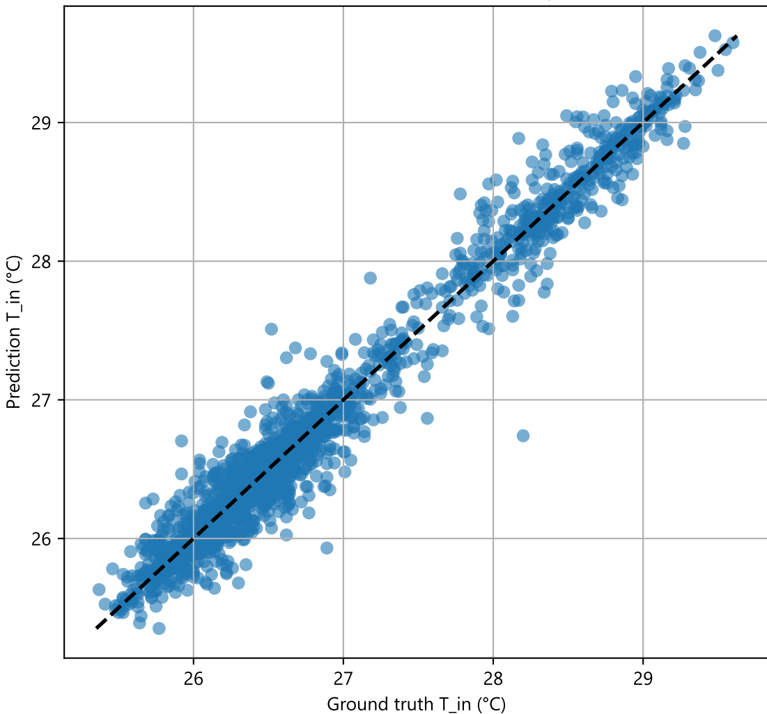
Ground Truth vs Prediction — Temperature ( T_{in} ) Quantized INT8 Conv1D Tiny
