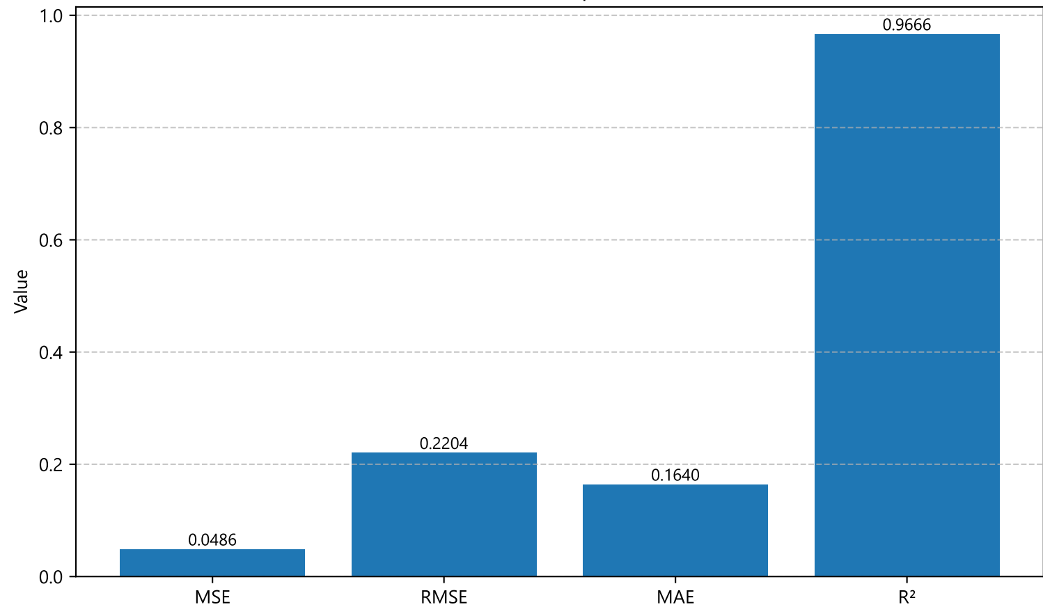
Evaluation metrics - INT8-quantized LSTM model
