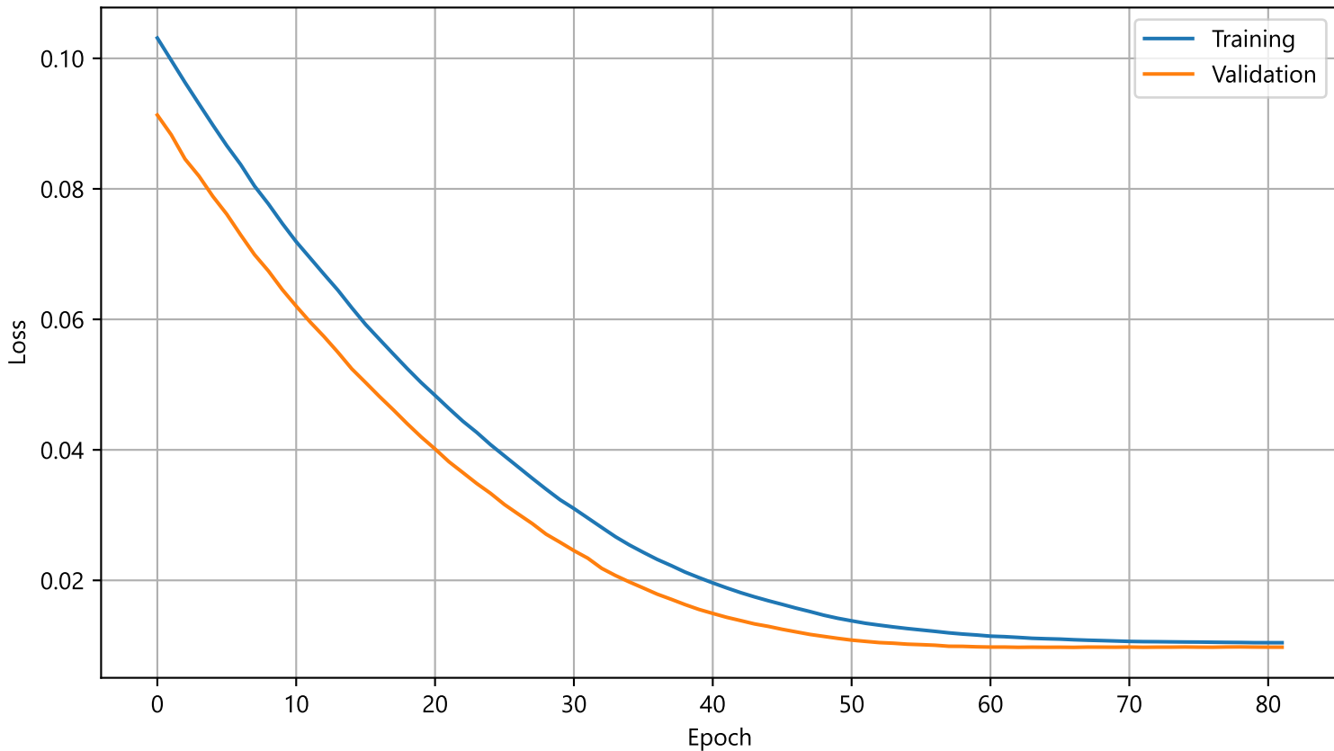
Training and validation loss during QAT (LSTM) Well-fitted model (generalization gap < 10%)
