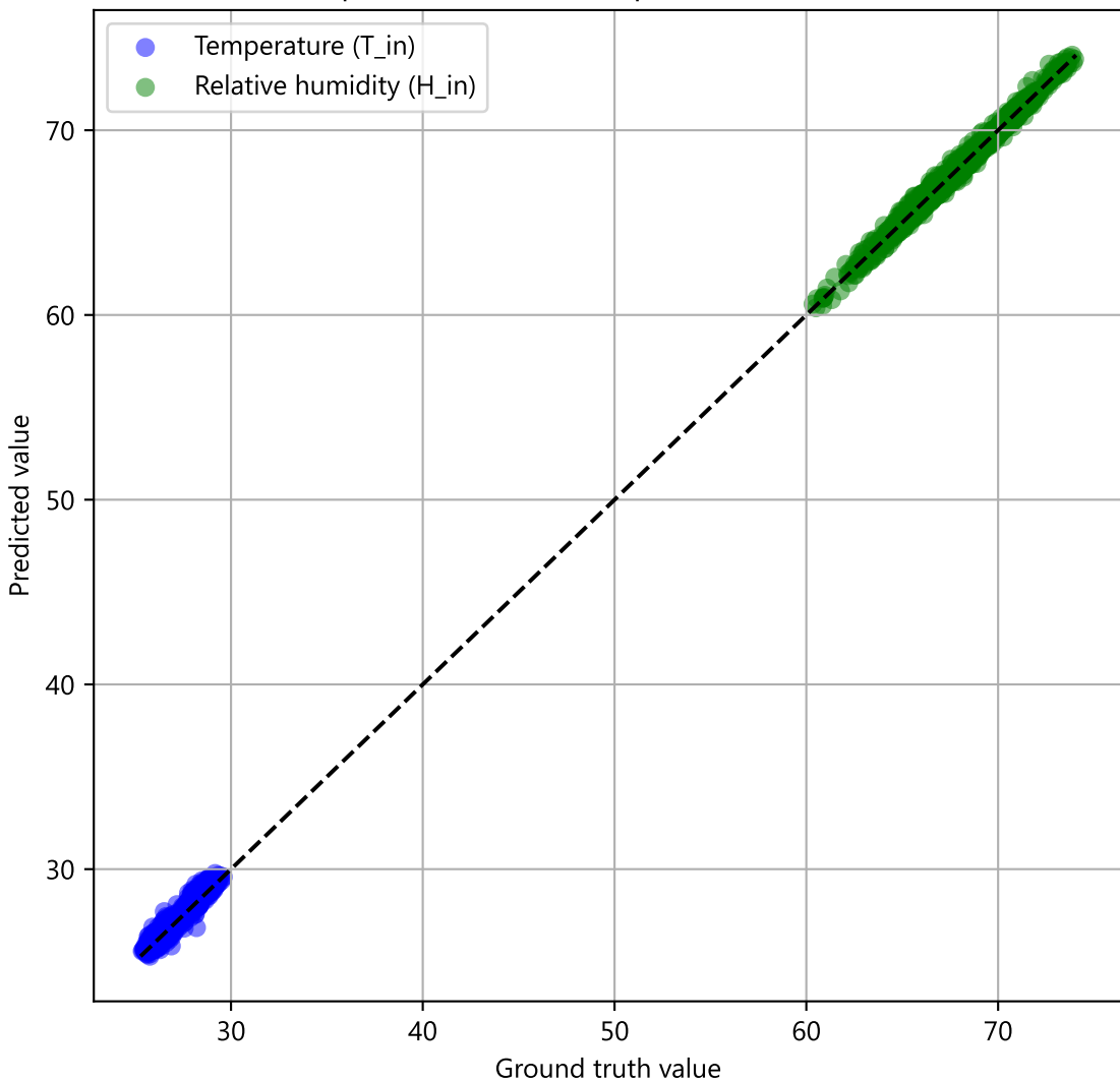
Joint prediction scatter - quantized LSTM model
