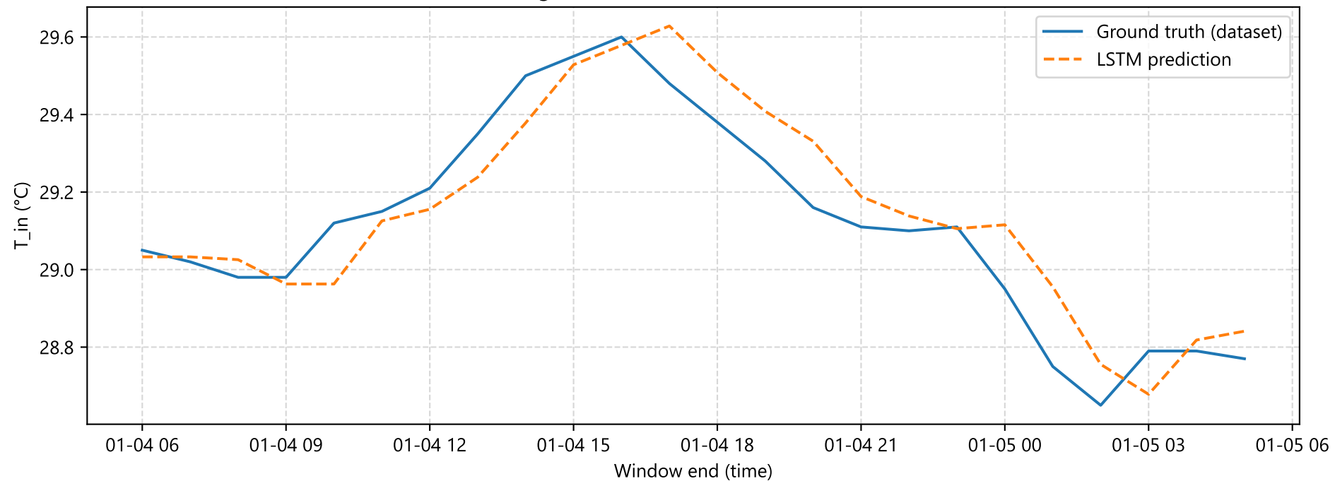
Rolling(24): T_in time series (window ends)
