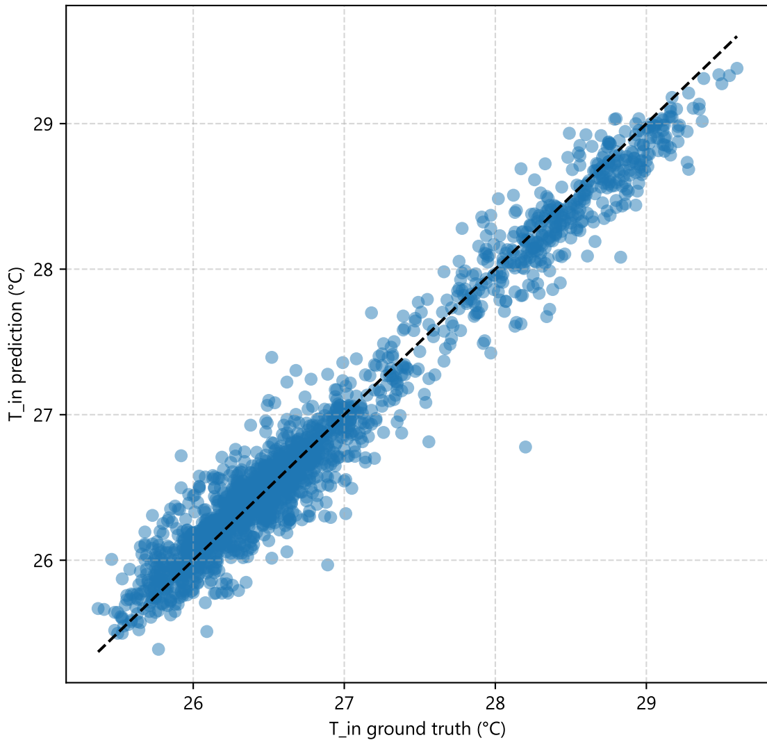
Scatter: ground truth vs prediction (T_in)
