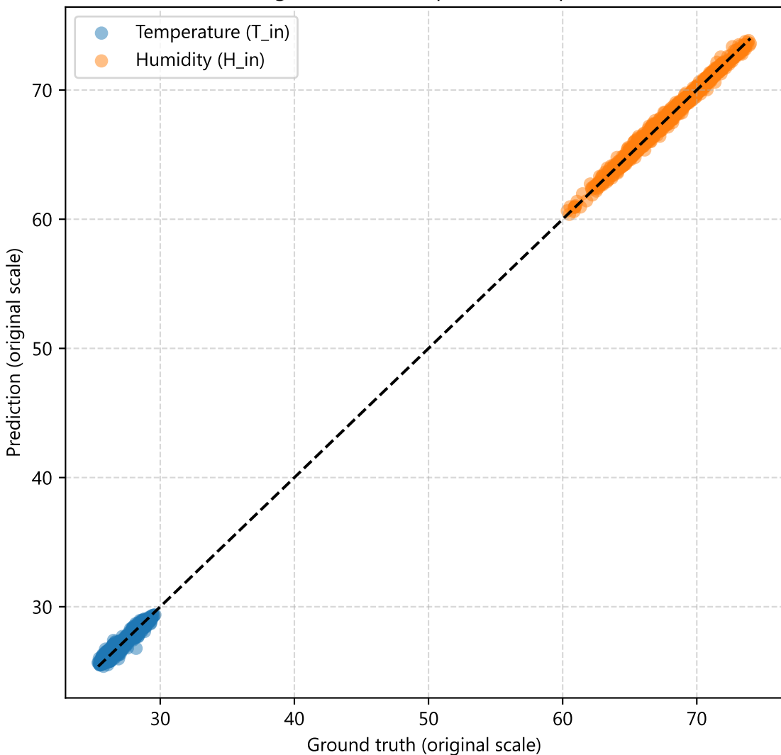
Joint scatter: ground truth vs prediction (quantized MLP)
