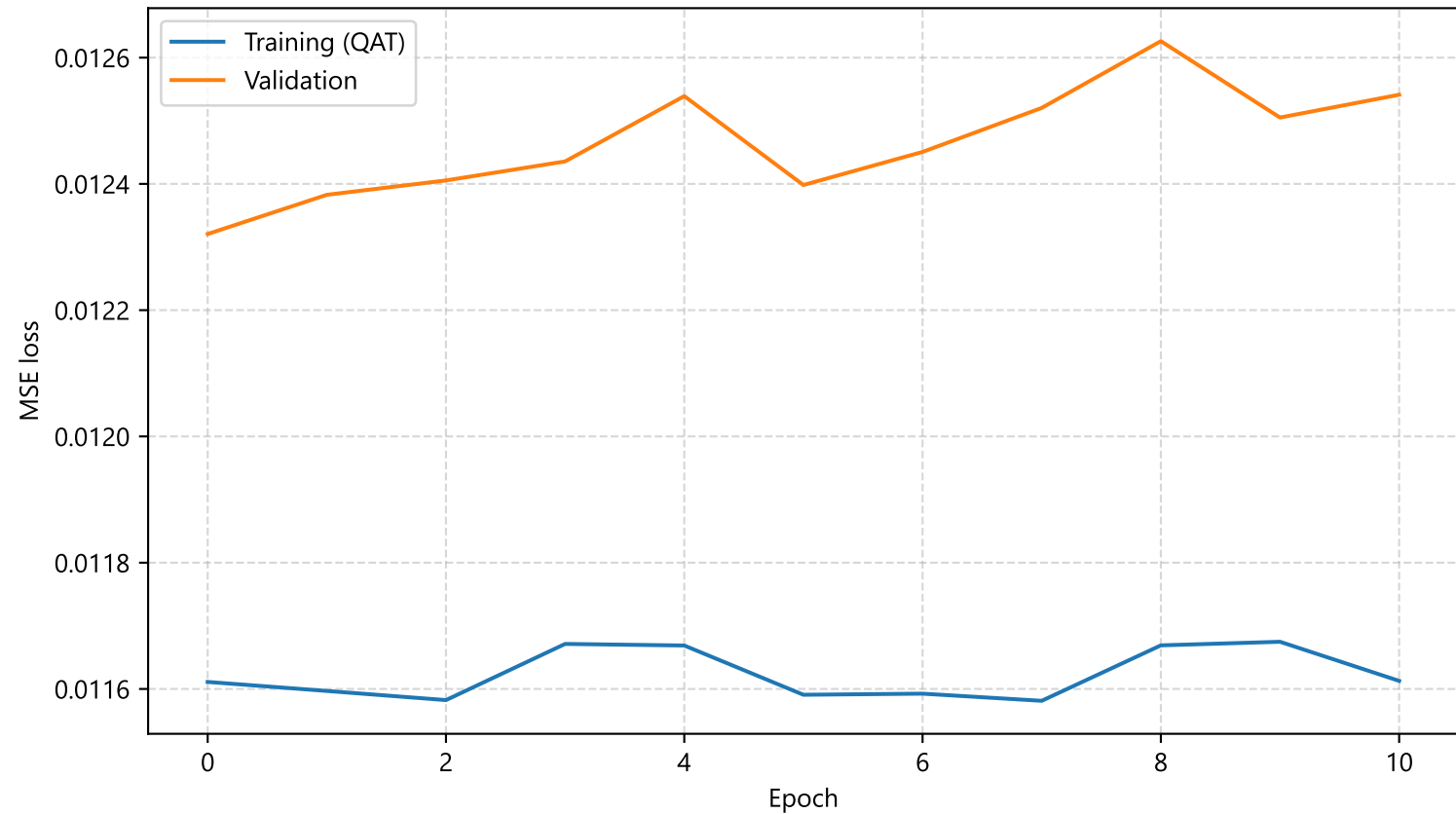
QAT training and validation loss Well-fitted model (generalization gap < 10%)
