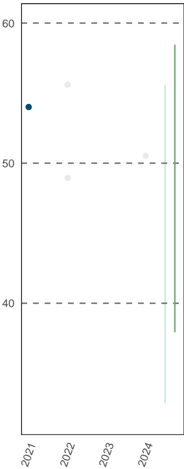
Northern ronquil
