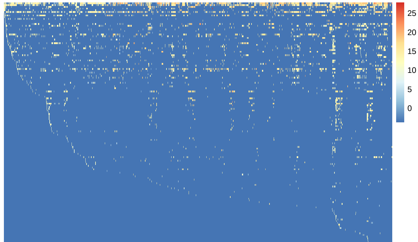
Taxa with VST, DESeq2
