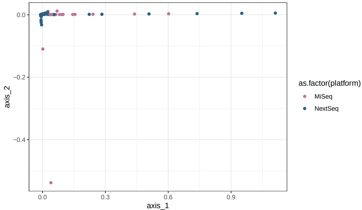
Wisconsin with vegan, by taxa
