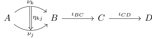
Diagram 1: Basic 2-Categorical Structure
