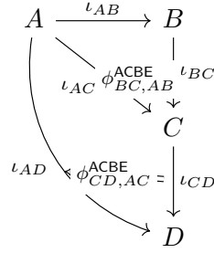
Figure 26.1: ACBE Pseudo-Functor Structure: The compositor 2-cells \phi^{\text{ACBE}} witness the isomorphism between staged descent and direct descent.
