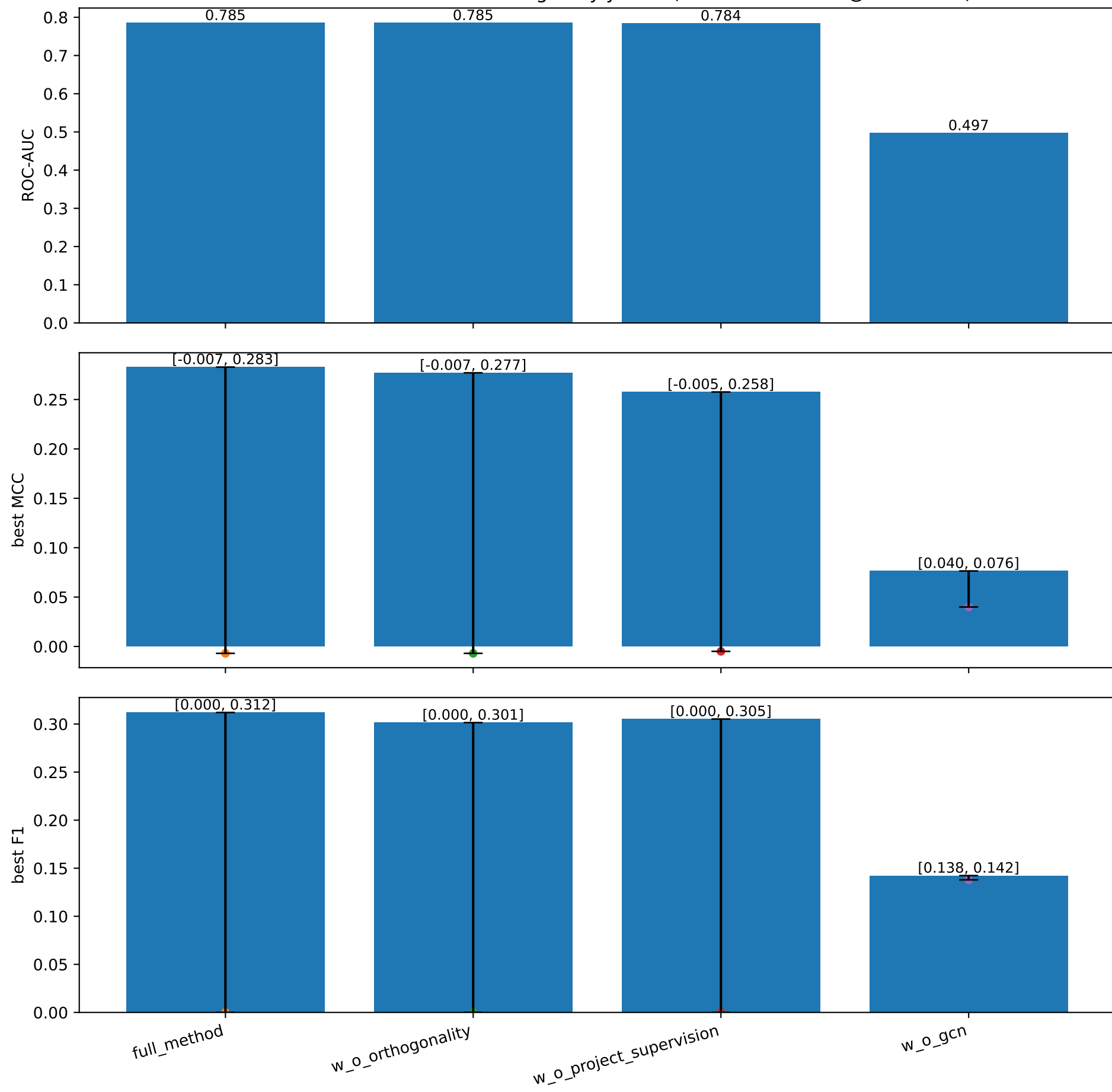
Zero-shot ablation metrics on target Mylyn-3.1 (interval = default@0.5 → best)
