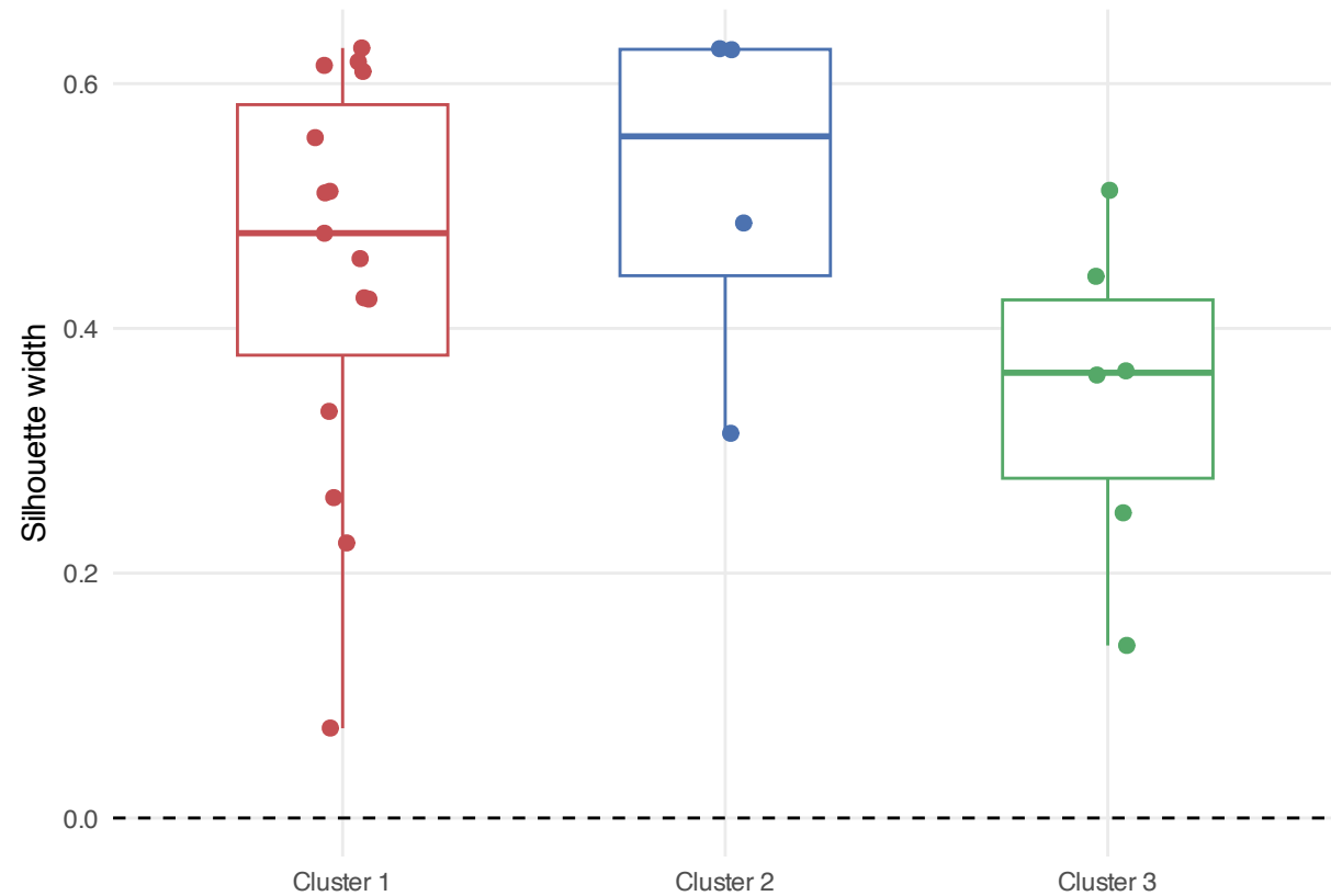
D. Baseline cluster-wise silhouette
