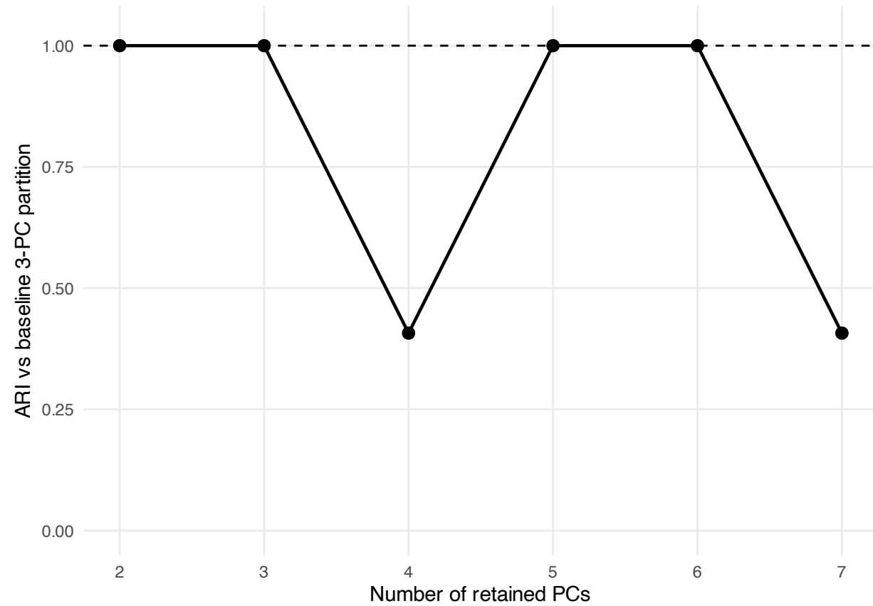
C. Sensitivity to retained PCA dimensionality
