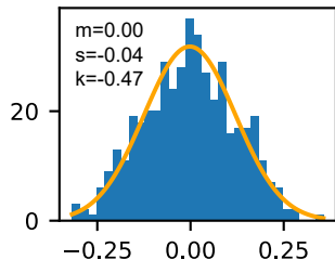
fc2.weight
