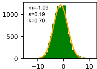
fc3.activation
