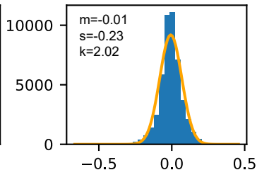
conv2.activation
