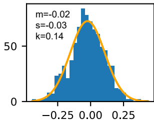
fc2.activation
