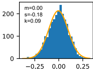
fc3.weight
