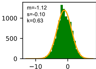
fc1.activation
