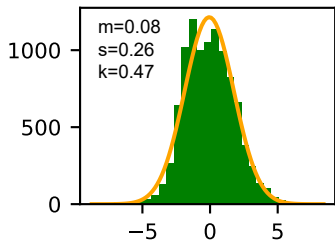
fc2.activation
